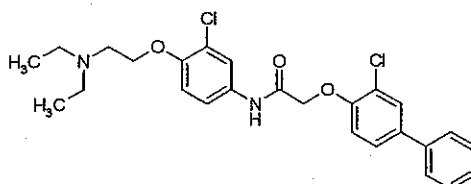
2-(3-chloro-biphenyl-4-yloxy)-N-[3-chloro-4-(2-diethylamino-ethoxy)-phenyl]-acetamide
