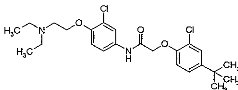
2-(4-tert.-butyl-2-chloro-phenoxy)-N-[3-chloro-4-(2-diethylamino-ethoxy)-phenyl]-acetamide
