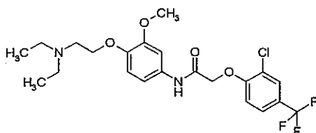
2-(2-chloro-4-trifluoromethyl-phenoxy)-N-[4-(2-diethylamino-ethoxy)-3-methoxy-phenyl]-acetamide
