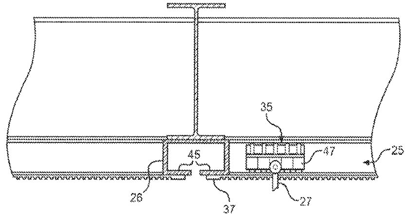
FIG. 4 PRIOR ART
