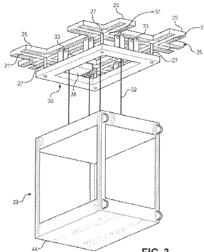
FIG. 3 PRIOR ART
