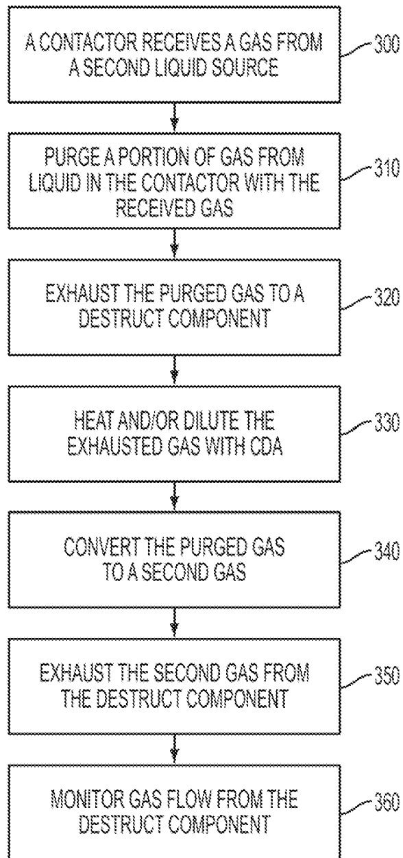
FIG. 2B (DEGASSING PROCESS)
