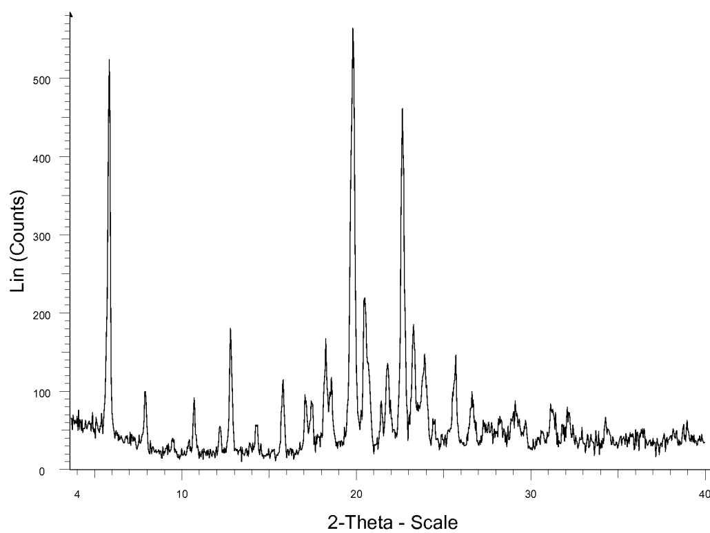
FIG. 1. X-ray powder diffraction pattern of Example 109-B.
