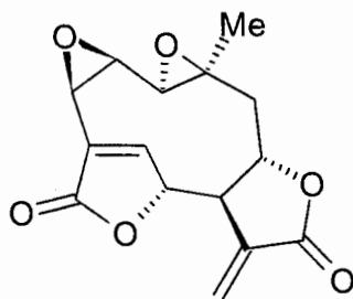
mikanolide
