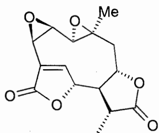
dihydromikanolide
