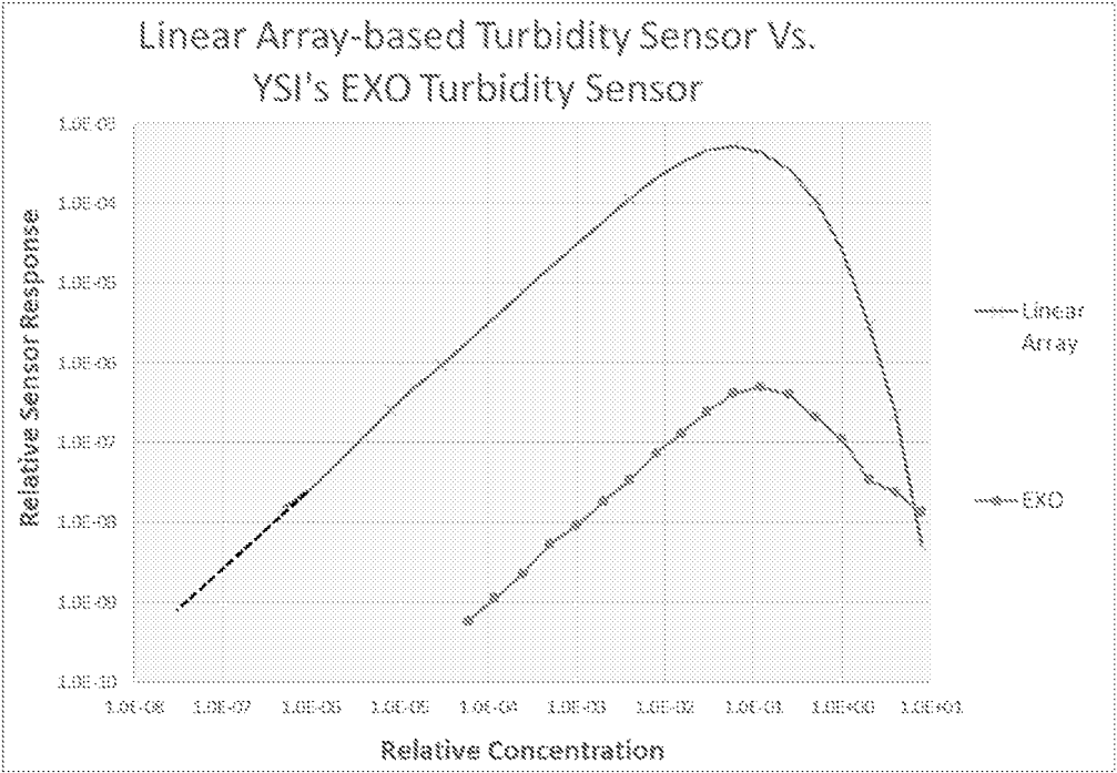
Figure 5: Sensitivity Comparison
