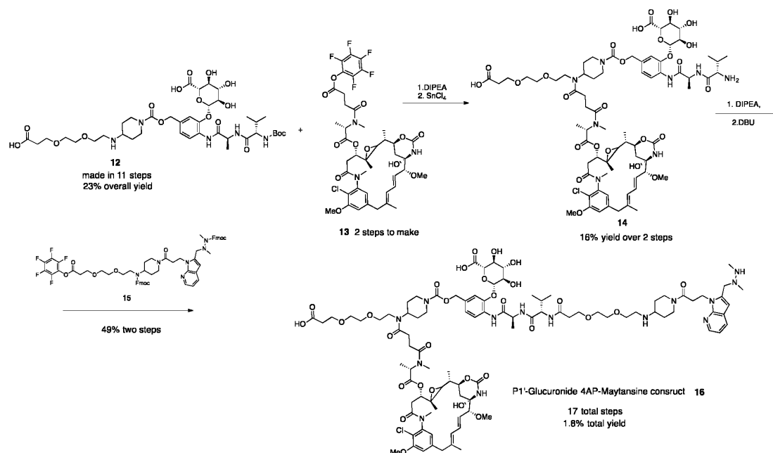
Scheme 2. Synthesis of P1'-glucuronide 4AP-Maytansine construct 16 .
