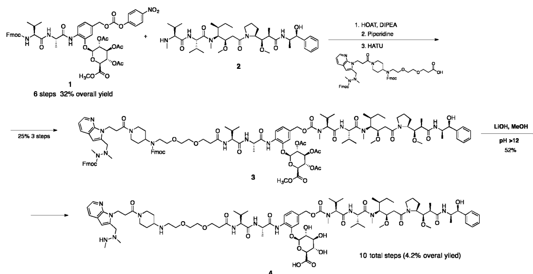
Scheme 1. P1'-Glucuronide dual-cleavage MMAE construct 4 .
