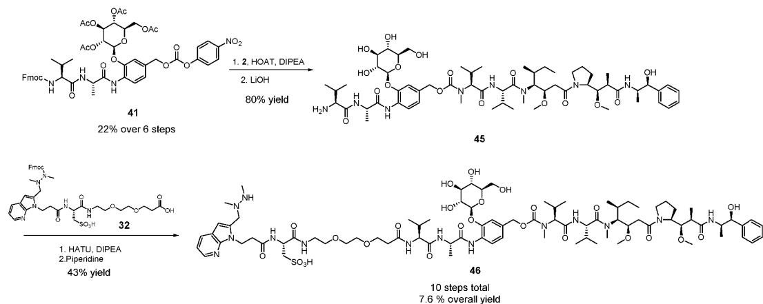
Scheme 7. Synthesis of glucoside MMAE construct 46 .
