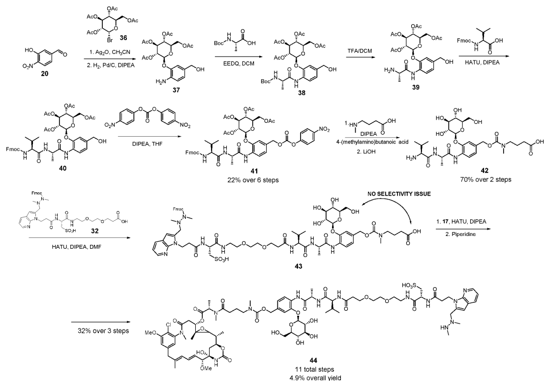
Scheme 5. Synthesis of P1'-glucoside NMC3-Maytansine construct 44 .
