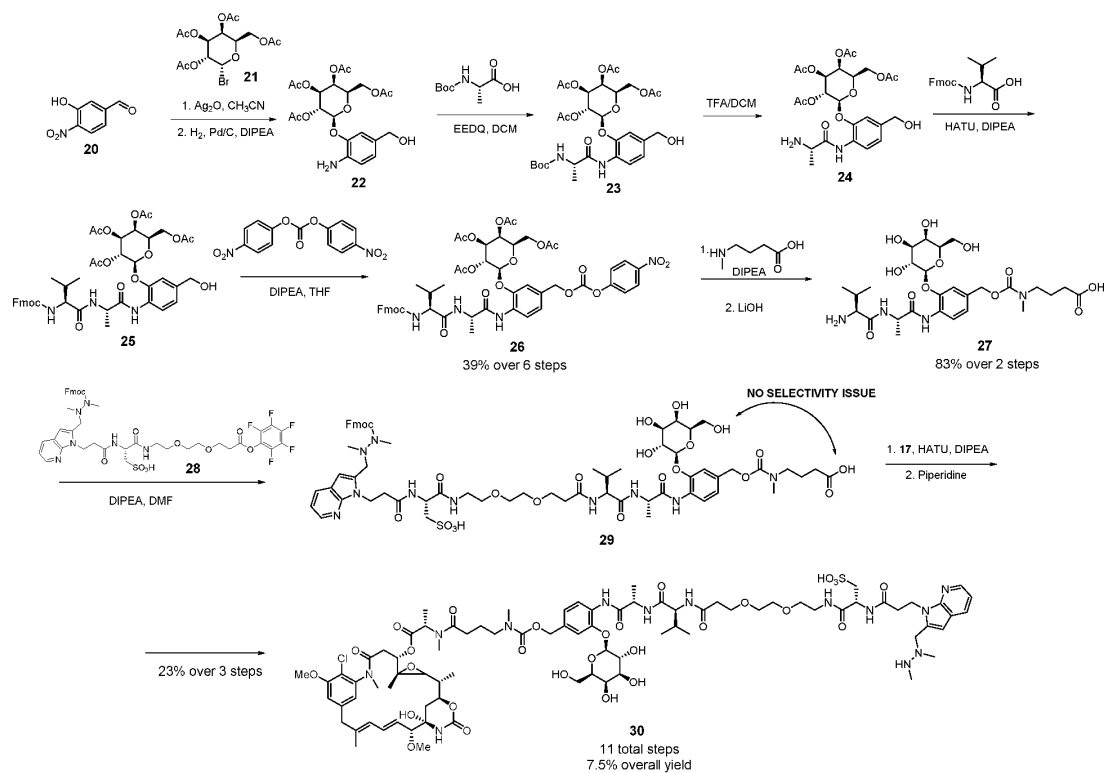
Scheme 4. Synthesis of P1'-galactoside NMC3-Maytansine construct 30 .
