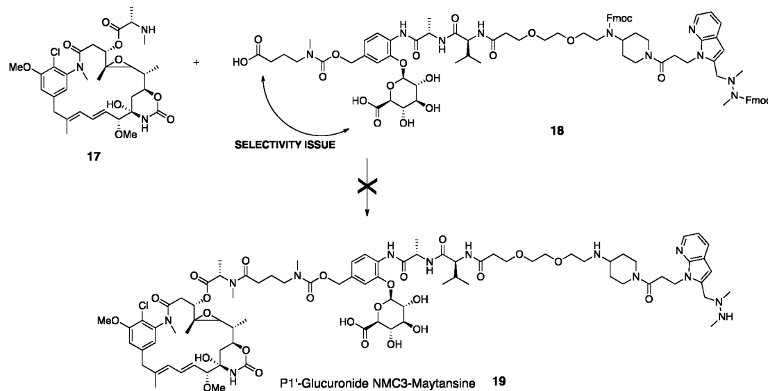
Scheme 3. Synthetic approach to P1'-Glucuronide NMC3-Maytansine construct 19 (not feasible due to the presence of free carboxylic acid in glucuronide moiety).
