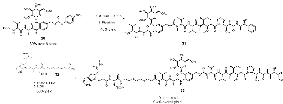
Scheme 6. Synthesis of P1'-galactoside MMAE construct 33 .
