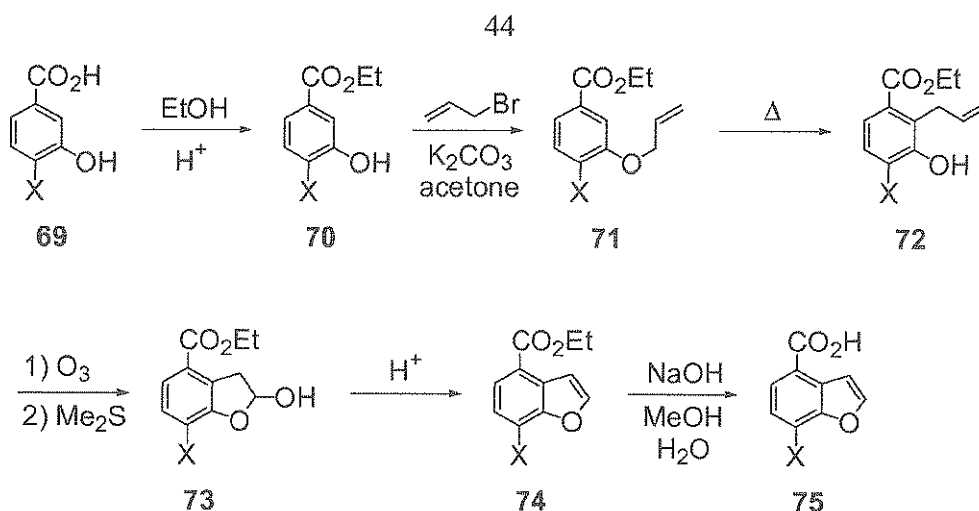
Scheme 10: Synthesis of benzofuran-carboxylic acid derivatives wherein X is fluorine or bromine
