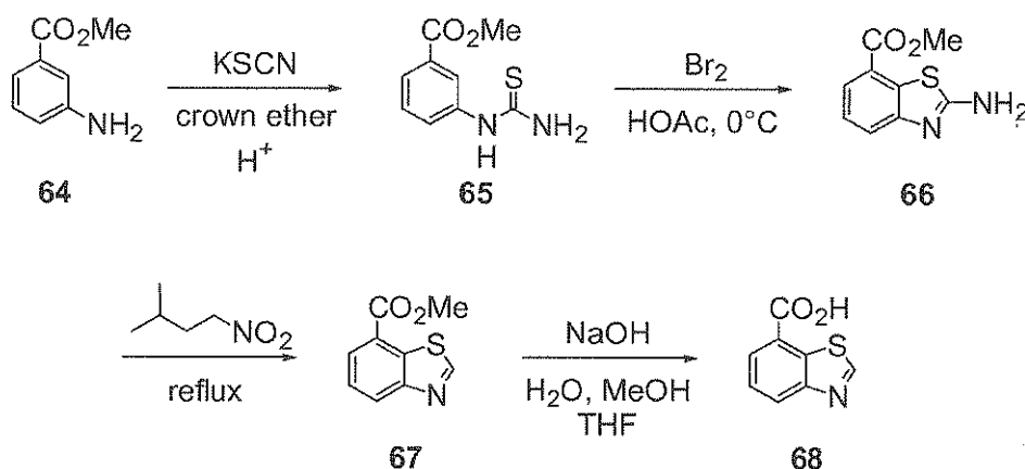
Scheme 9: Synthesis of benzothiazole-carboxylic acid derivatives
