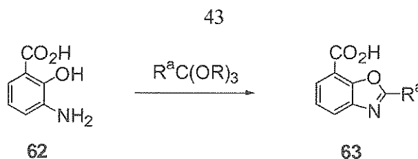
Scheme 8: Synthesis of benzoxazole-carboxylic acid derivatives wherein R is methyl or ethyl and R a is hydrogen or methyl
