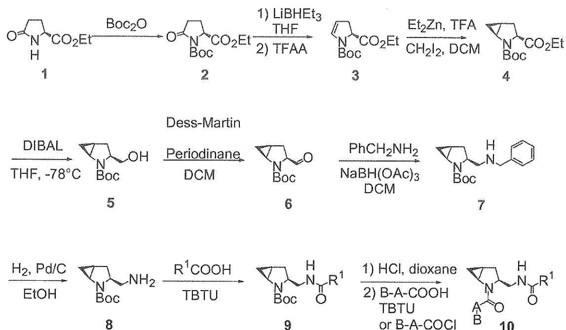
Scheme 1: Synthesis of compounds of formula (I) and/or (Ia)
