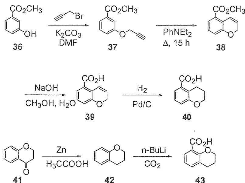
Scheme 6 : Synthesis of chroman-carboxylic acid derivatives
