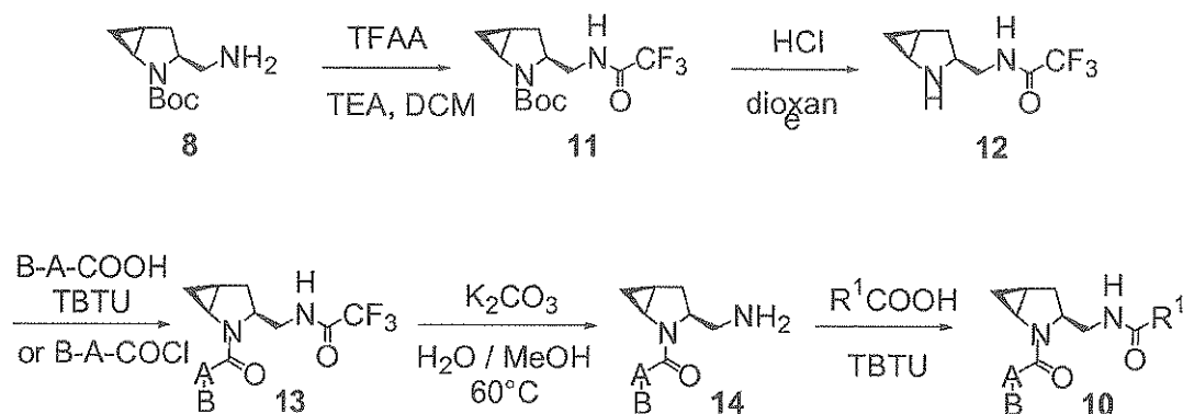
Scheme 2: Alternative synthesis of compounds of formula (I) and/or (Ia)
