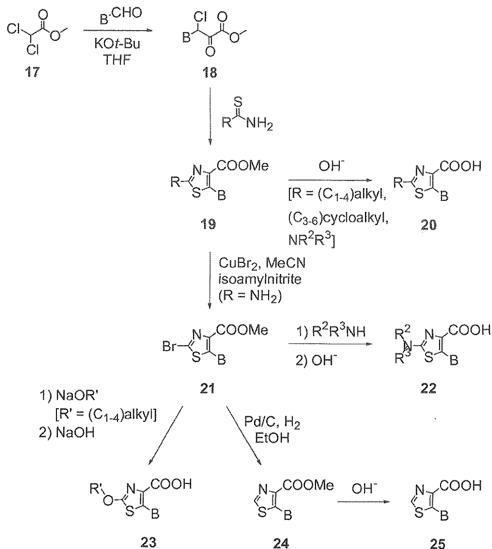
Scheme 4: Synthesis of thiazole-4-carboxylic acid derivatives, wherein R is (C 1-4 )alkyl, (C 3-6 )cycloalkyl or NR 2 R 3 and R' is (C 1-4 )alkyl
