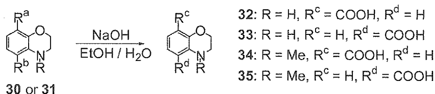
Scheme 5 : Synthesis of benzo[1,4]oxazine-carboxylic acid derivatives
