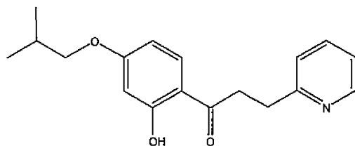
1-(2-hydroxy-4-isobutoxyphenyl)-3-(pyridine-2-yl)propan-1-one.
