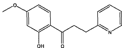
1-(2-hydroxy-4-isobutoxyphenyl)-3-(pyridine-2-yl)propan-1-one.
