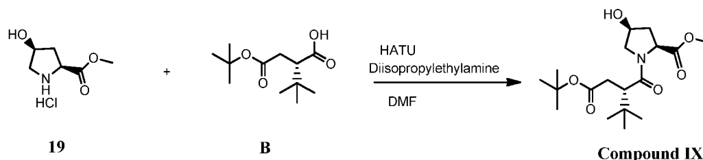
Scheme IX
