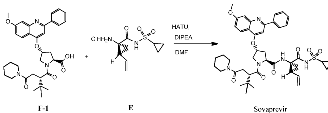
Scheme XIII
