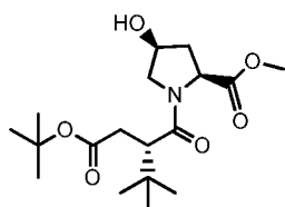
Compound IX.
