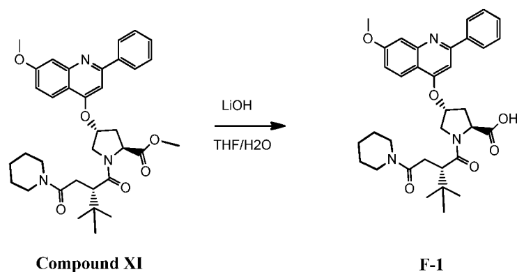
Scheme XII
