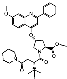
Compound XI.
