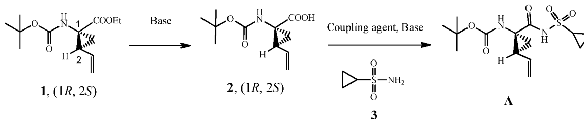
Scheme I
