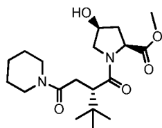
Compound X.
