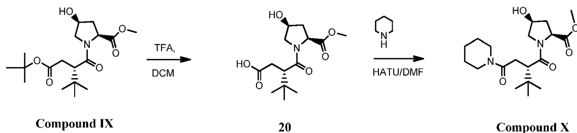
Scheme X
