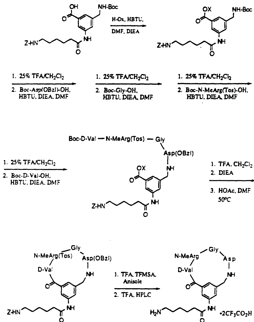
Scheme 16
