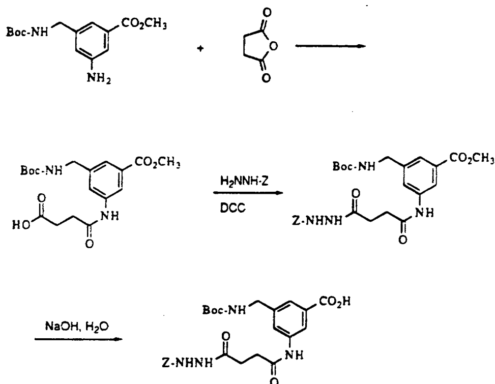
Scheme 12
