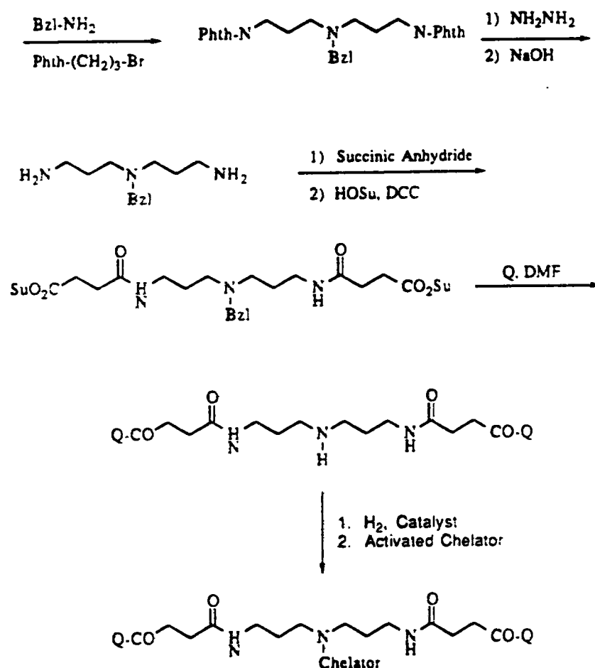
Scheme 33
