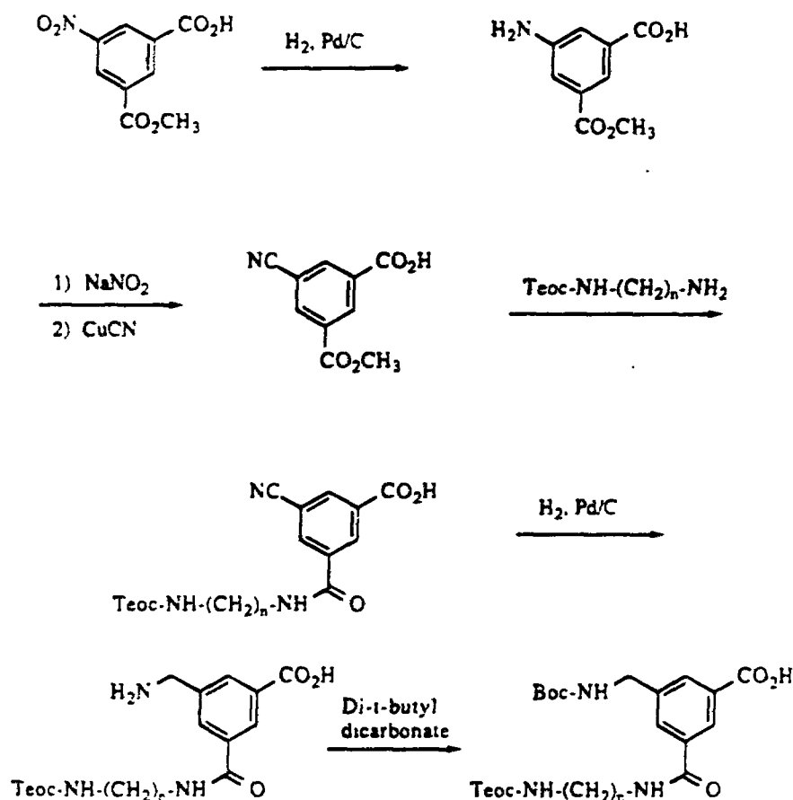
Scheme 10
