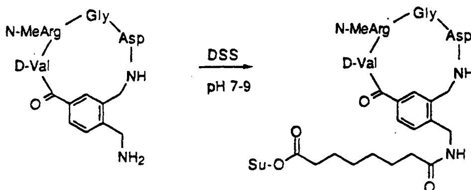
Scheme 18
