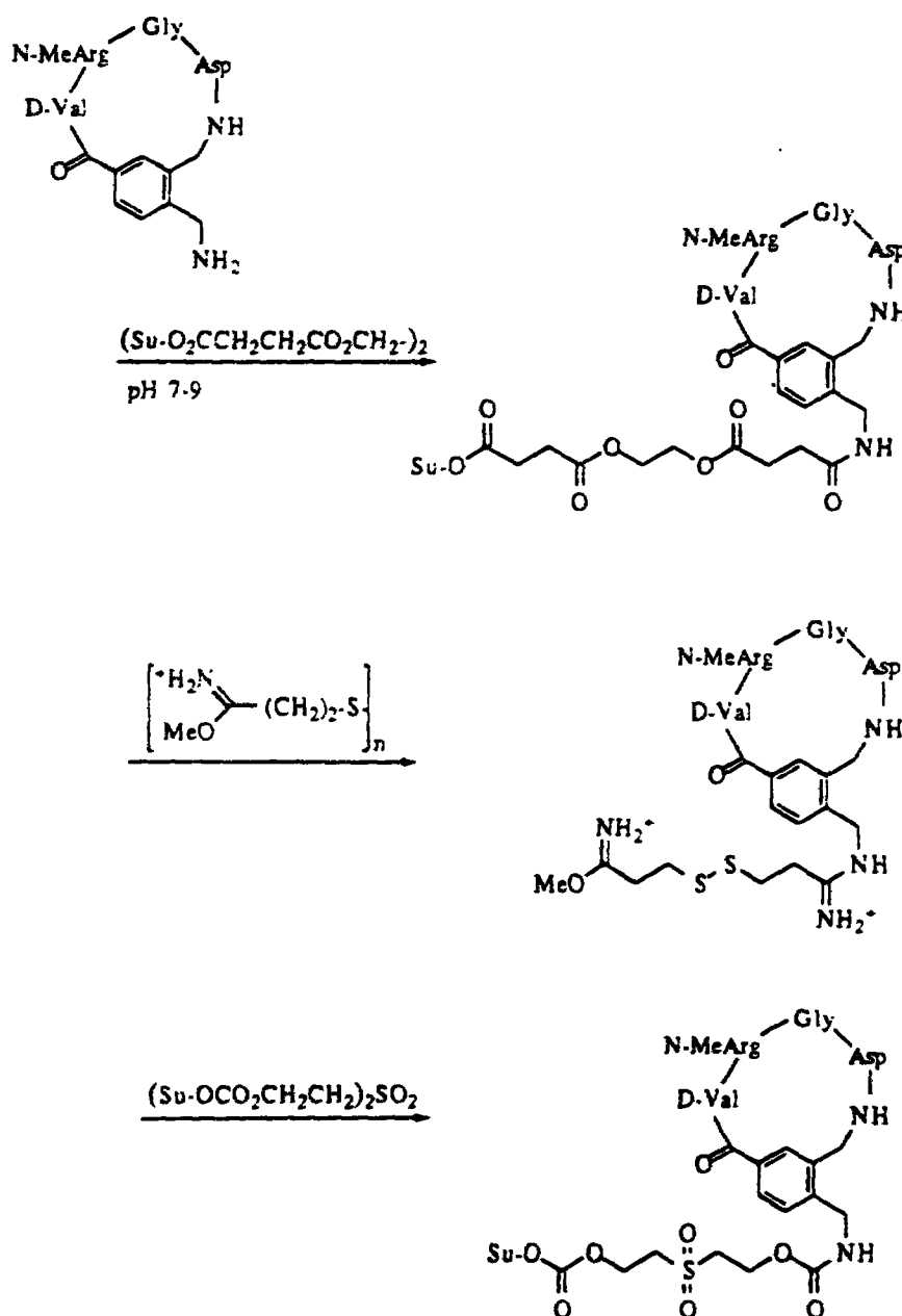
Scheme 20
