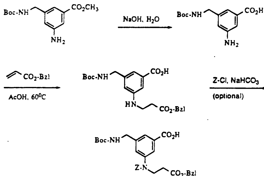
Scheme 8
