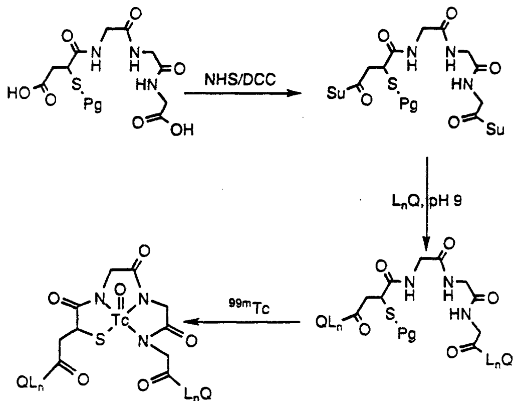
Scheme 28
