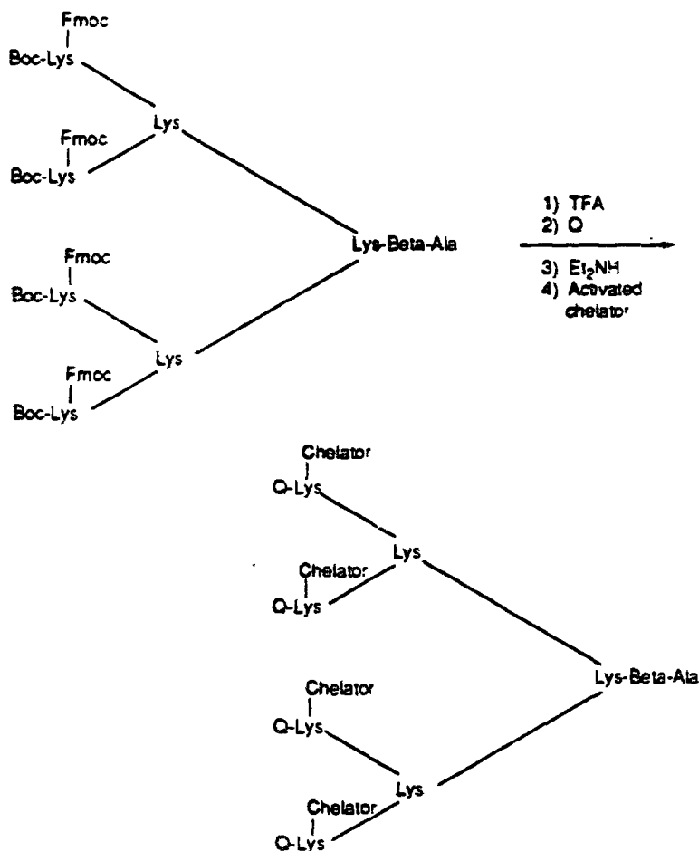
Scheme 35
