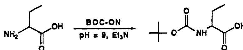
D-2-aminobutyric acid
