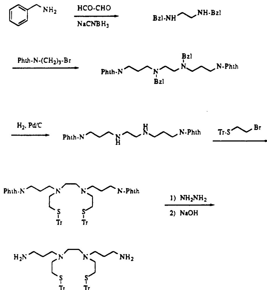
Scheme 32
