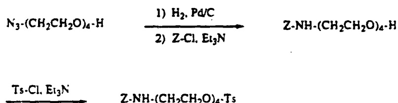
Scheme 14
