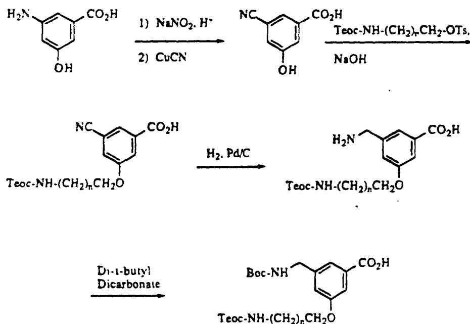
Scheme 11
