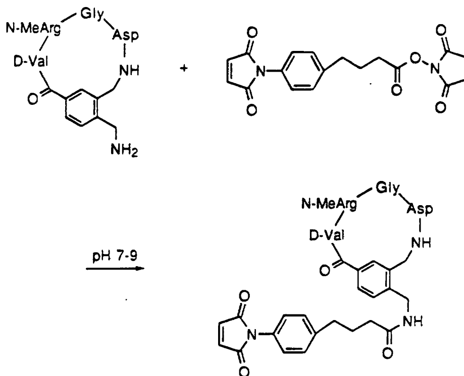
Scheme 19
