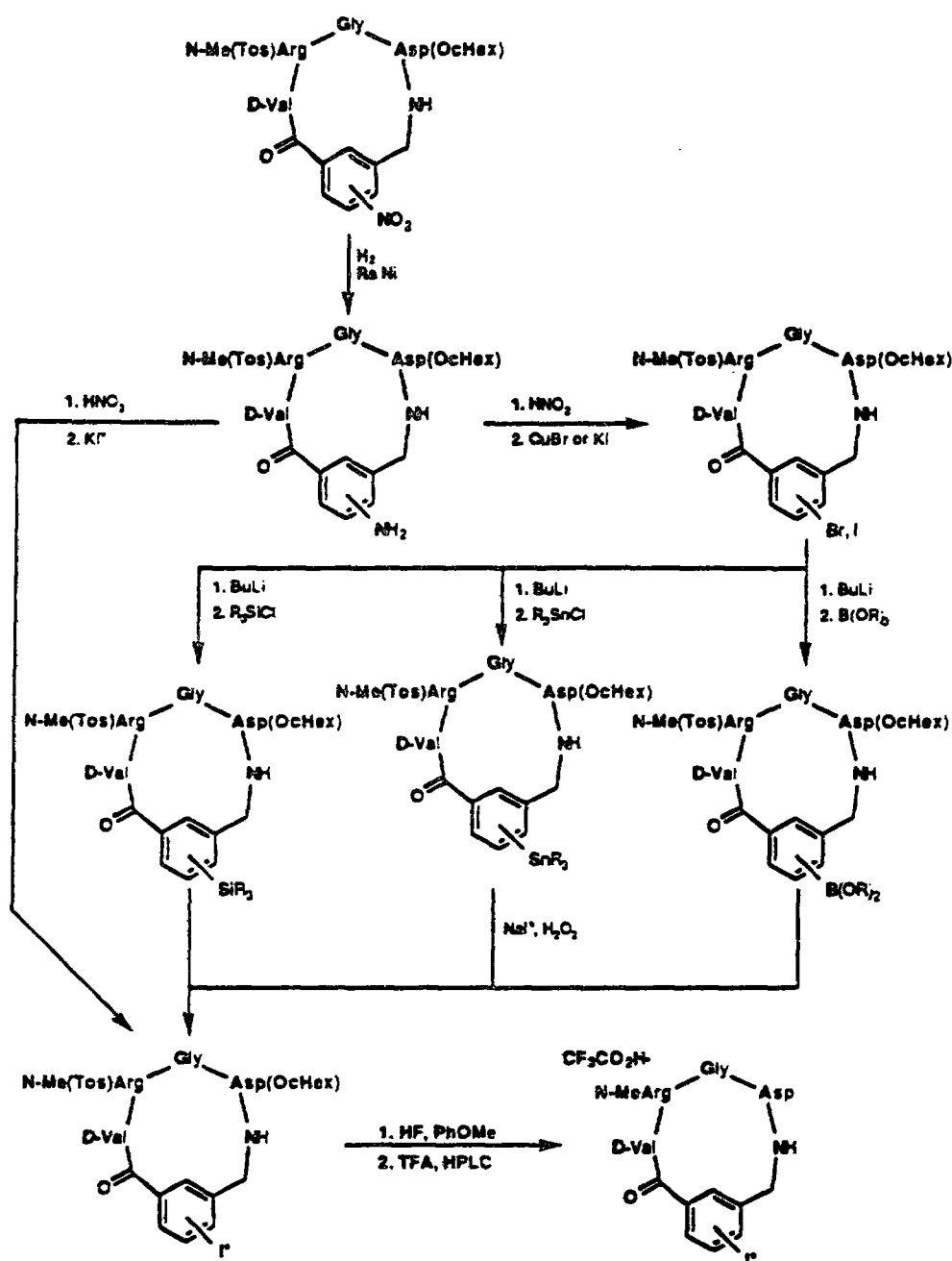
Scheme 38
