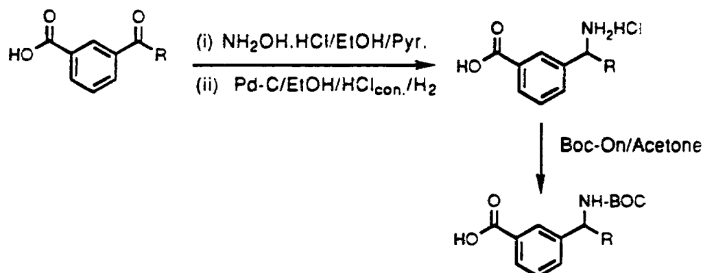
Scheme 4:
