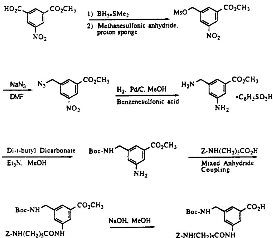
Scheme 9
