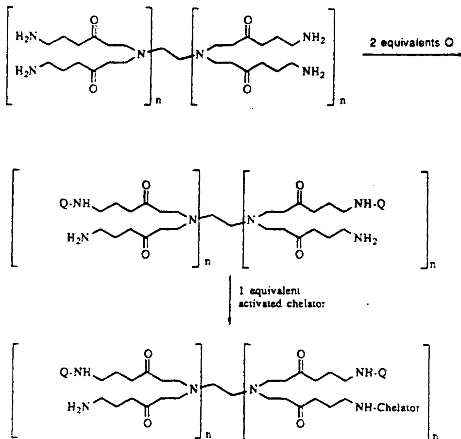
Scheme 34
