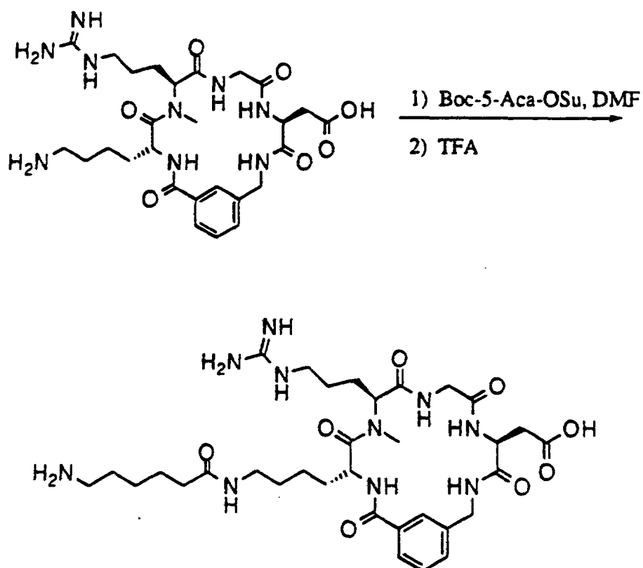
Scheme 17
