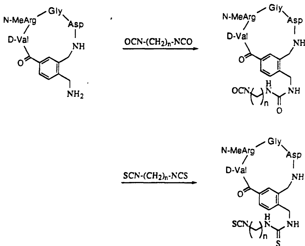
Scheme 21
