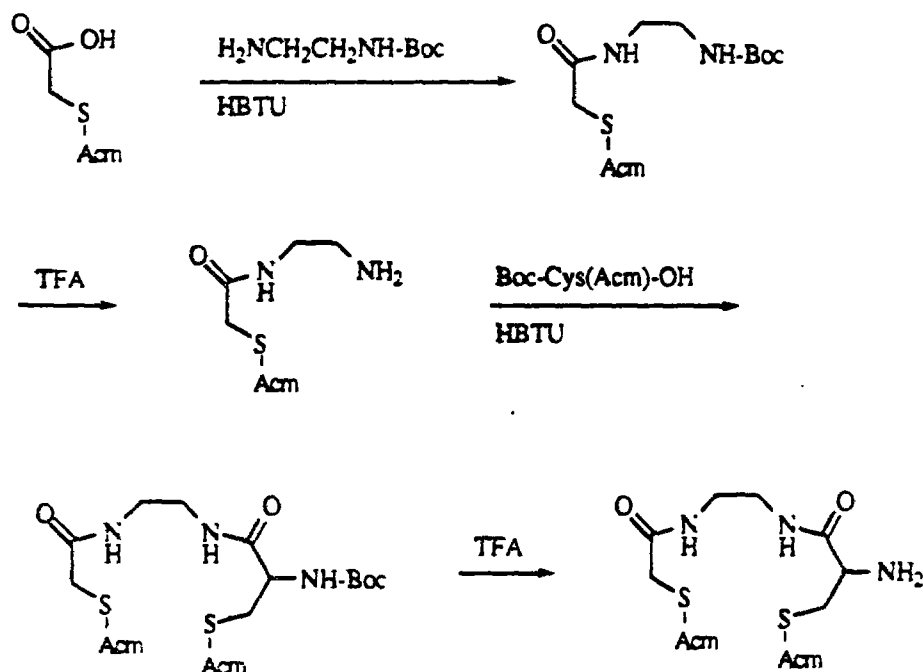
Scheme 27
