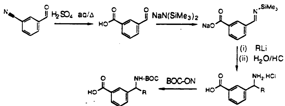
10 Scheme 2:
