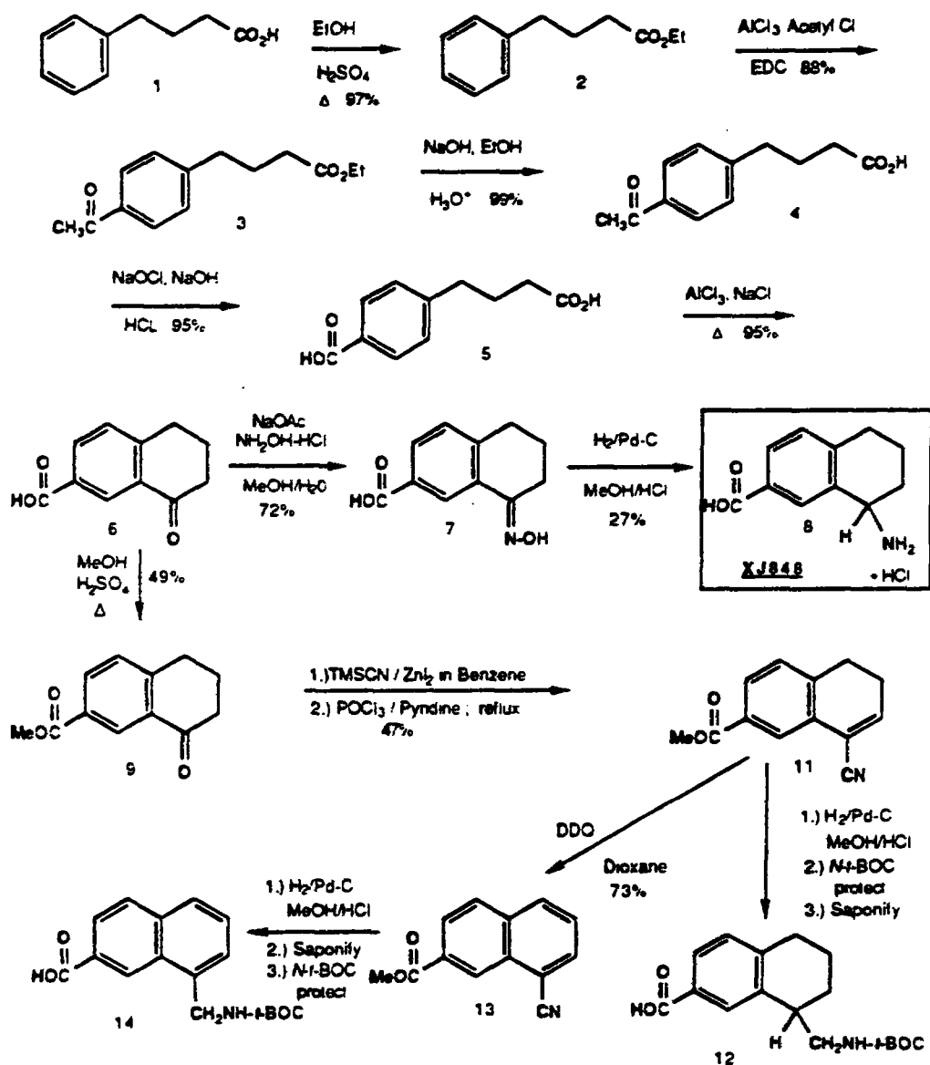
Scheme 7
