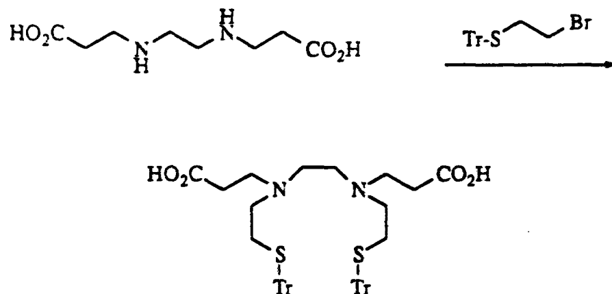
Scheme 31
