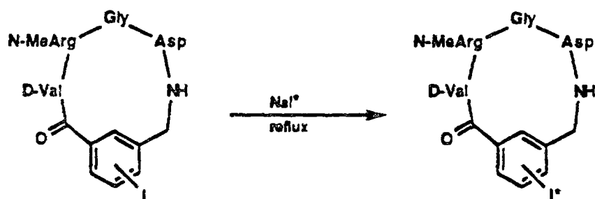
Scheme 37
