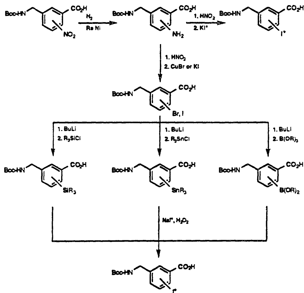
Scheme 36
