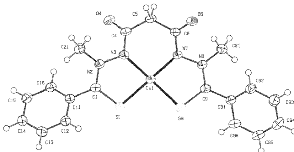
ORTEP diagram of compound 1 showing 50% thermal ellipsoids.
