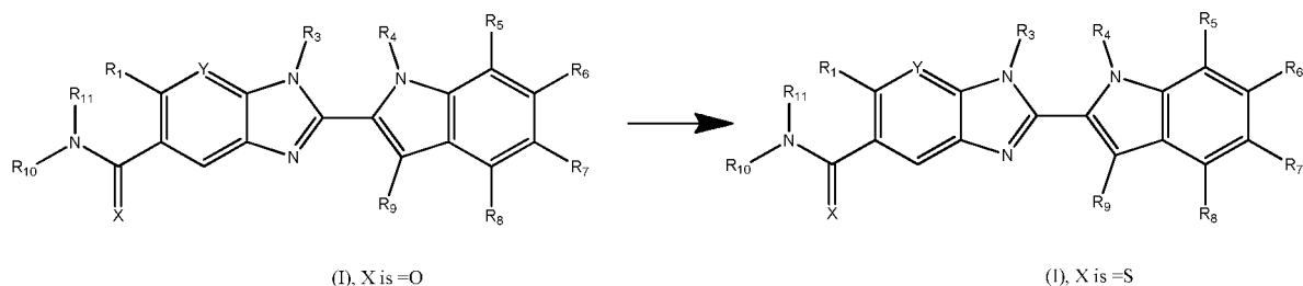
Scheme 10
