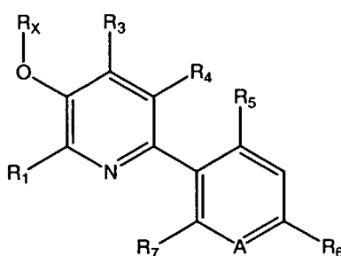
Formula IX
