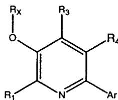
Formula VIII
