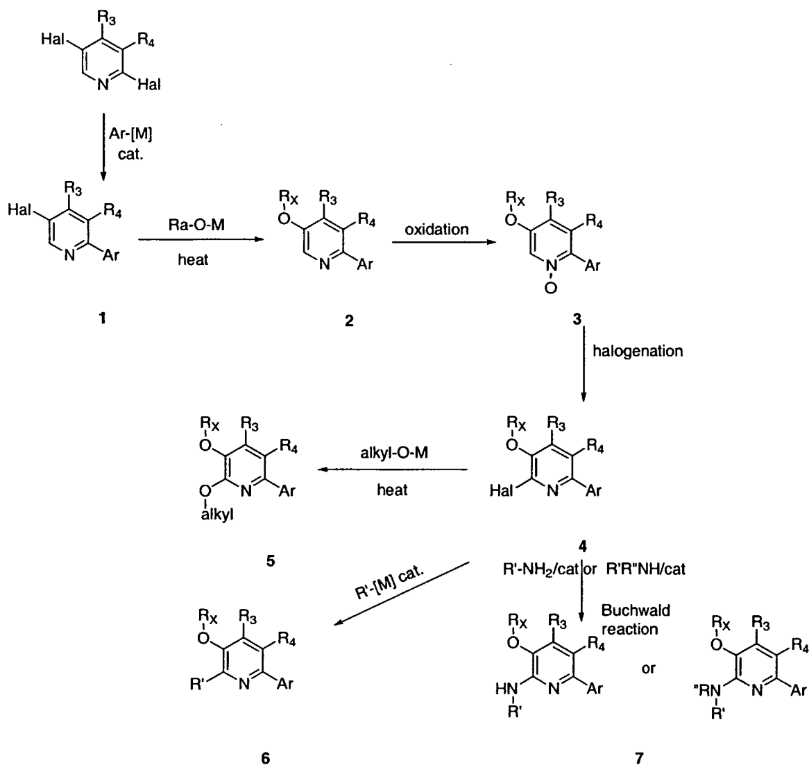
Scheme I
