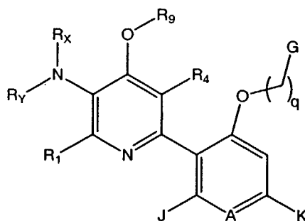
Formula VII
