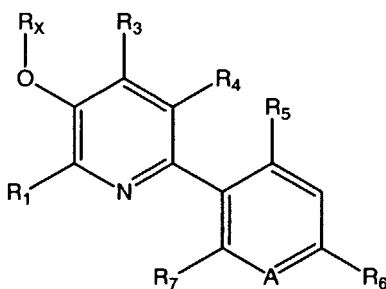
Formula IX
