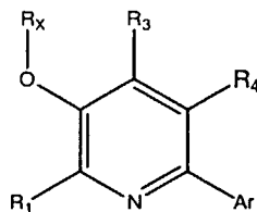
Formula VIII
