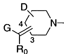
Formula X-c
