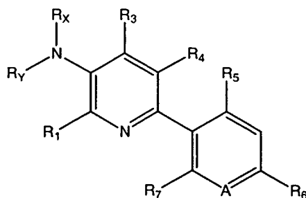
Formula III
