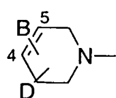
Formula X-a
