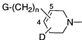
Formula X-b
