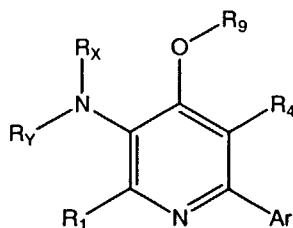
Formula V
