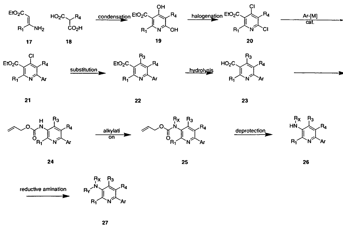
Scheme III
