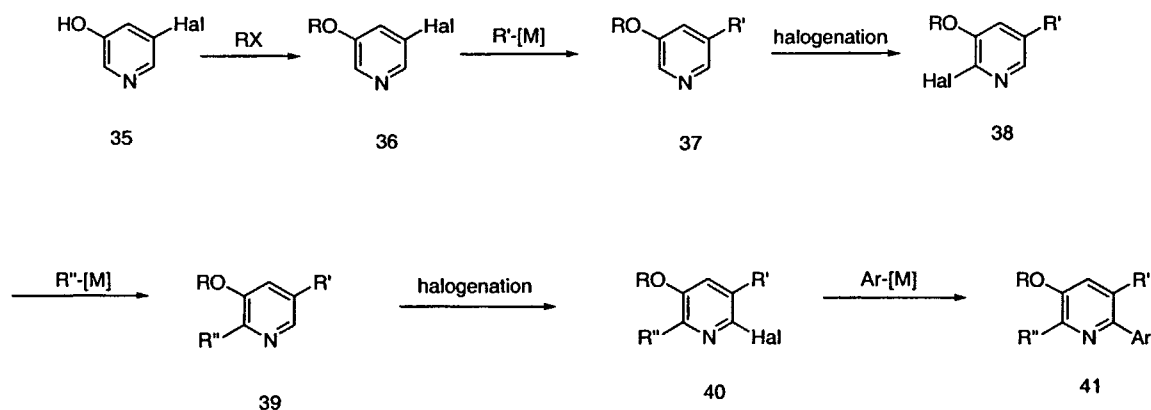
Scheme V
