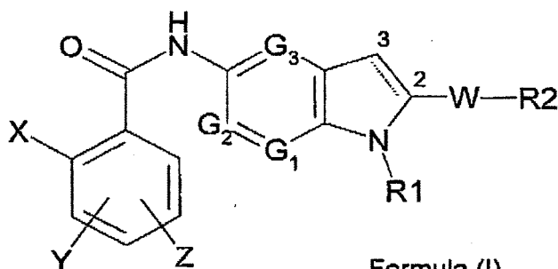
Formula (I)
