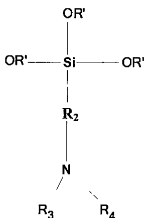
Formula (II)
