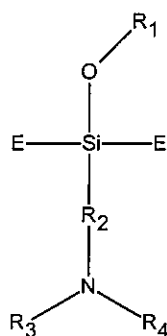
Formula (I)
