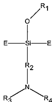
Formula (I)
