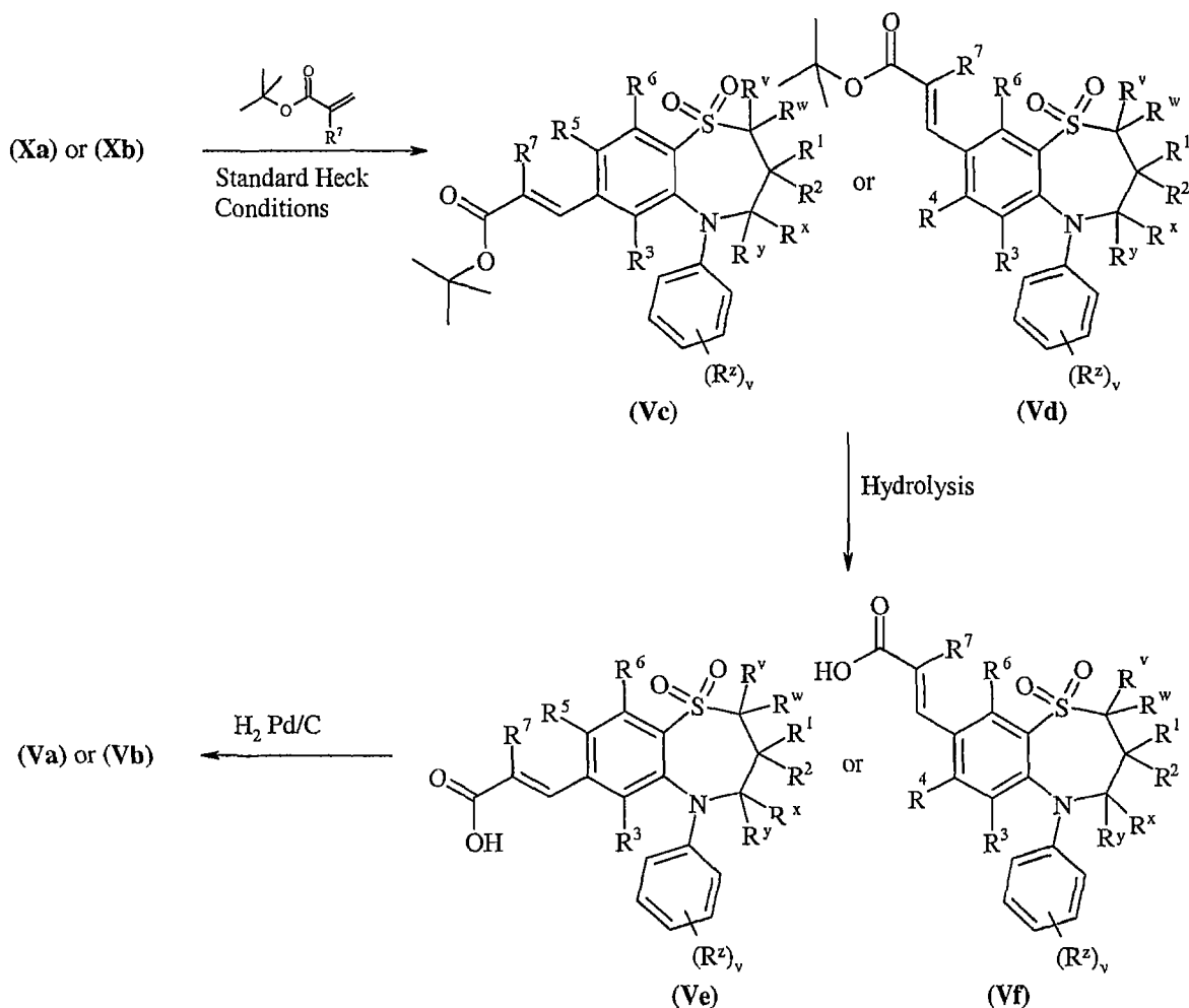
Scheme 3
