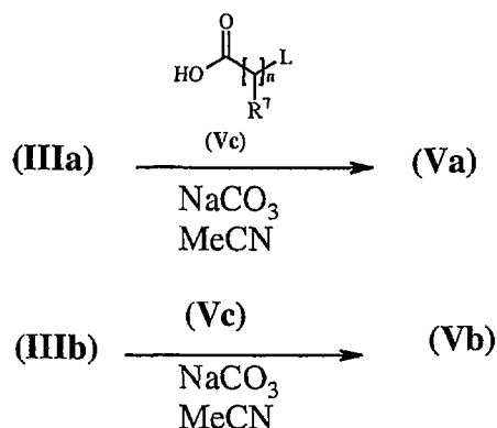
Scheme 2
