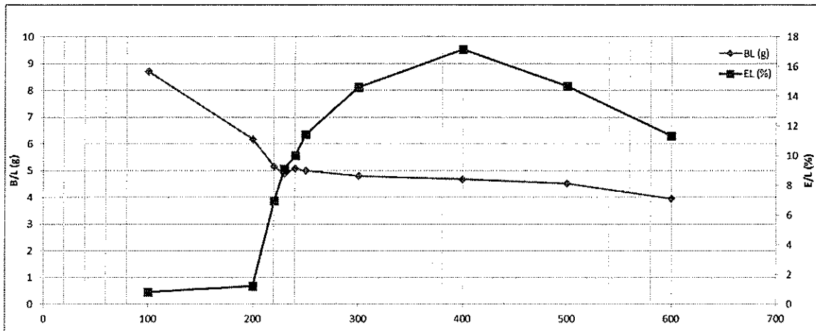
Fig.1 Annealing curve of a wire (sample 1, Table 1)
