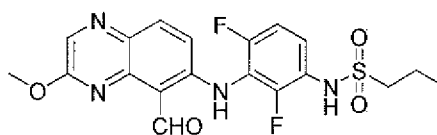
N -(2,4-difluoro-3-(5-formyl-3-methoxyquinoxalin-6-ylamino)phenyl)propane-1-sulfonamide
