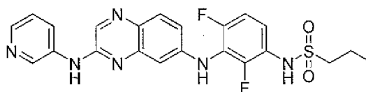
N1-(2,4-difluoro-3-[[3-(3-pyridylamino)-6-quinoxaliny]amino]phenyl)-1-propanesulfonamide
