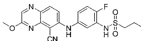
N -(5-(5-cyano-3-methoxyquinoxalin-6-ylamino)-2-fluorophenyl)propane-1-sulfonamide
