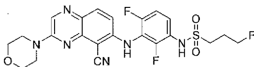
N -(3-(5-cyano-3-morpholinoquinoxalin-6-ylamino)-2,4-difluorophenyl)-3-fluoropropane-1-sulfonamide
