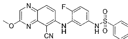
N -(3-(5-cyano-3-methoxyquinoxalin-6-ylamino)-4-fluorophenyl)benzenesulfonamide
