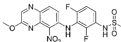
N-(2,4-difluoro-3-[[3-(methoxy-5-nitro-6-quinoxaliny]amino]phenyl) methanesulfonamide
