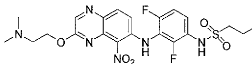
N1-(3-((3-(2-(dimethylamino)ethoxy)-5-nitro-6-quinoxaliny)amino)-2,4-difluorophenyl)-1-propanesulfonamide
