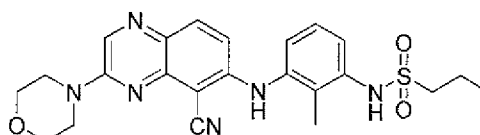
N -(3-(5-cyano-3-morpholinoquinoxalin-6-ylamino)-2-methylphenyl)propane-1-sulfonamide
