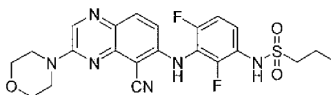
N -(3-(5-cyano-3-morpholinoquinoxalin-6-ylamino)-2,4-difluorophenyl)propane-1-sulfonamide
