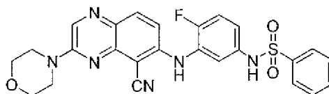
N -(3-(5-cyano-3-morpholinoquinoxalin-6-ylamino)-4-fluorophenyl)benzenesulfonamide
