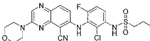
N -(2-chloro-3-(5-cyano-3-morpholinoquinoxalin-6-ylamino)-4-fluorophenyl)propane-1-sulfonamide
