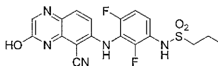
N1-(3-[[5-cyano-3-hydroxy-6-quinoxaliny]amino]-2,4-difluorophenyl)-1-propanesulfonamide
