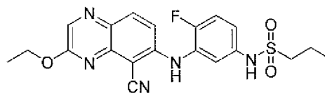
N -(3-(5-cyano-3-ethoxyquinoxalin-6-ylamino)-4-fluorophenyl)propane-1-sulfonamide
