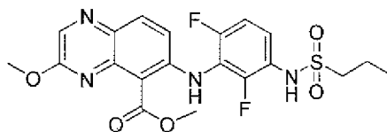
methyl 6-(2,6-difluoro-3-(propylsulfonamido)phenylamino)-3-methoxyquinoxaline-5-carboxylate
