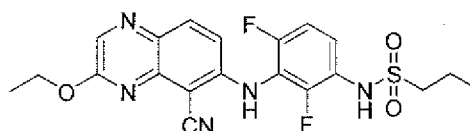
N-(3-(5-cyano-3-ethoxyquinoxalin-6-ylamino)-2,4-difluorophenyl)propane-1-sulfonamide
