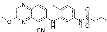
N -(3-(5-cyano-3-methoxyquinoxalin-6-ylamino)-4-methylphenyl)propane-1-sulfonamide
