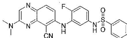
N -(3-(5-cyano-3-(dimethylamino)quinoxalin-6-ylamino)-4-fluorophenyl)benzenesulfonamide
