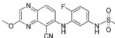
N -(3-(5-cyano-3-methoxyquinoxalin-6-ylamino)-4-fluorophenyl)methanesulfonamide
