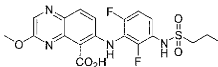
6-(2,6-difluoro-3-(propylsulfonamido)phenylamino)-3-methoxyquinoxaline-5-carboxylic acid
