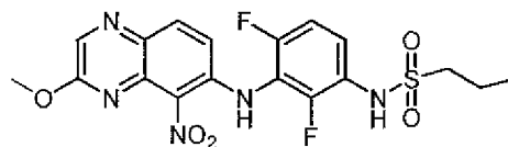
N1-(2,4-difluoro-3-((3-methoxy-5-nitro-6-quinoxaliny)amino)phenyl)-1-propanesulfonamide
