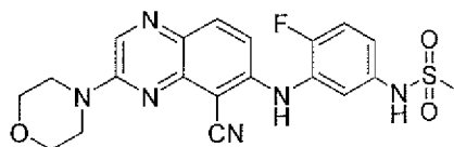
N -(3-(5-cyano-3-morpholinoquinoxalin-6-ylamino)-4-fluorophenyl)methanesulfonamide
