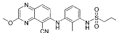
N -(3-(5-cyano-3-methoxyquinoxalin-6-ylamino)-2-methylphenyl)propane-1-sulfonamide
