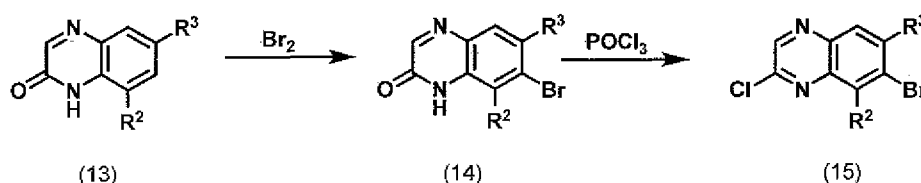
Reaction Scheme 4.
