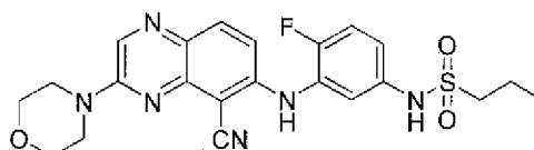
N -(3-(5-cyano-3-morpholinoquinoxalin-6-ylamino)-4-fluorophenyl)propane-1-sulfonamide
