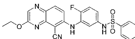
N -(3-(5-cyano-3-ethoxyquinoxalin-6-ylamino)-4-fluorophenyl)benzenesulfonamide
