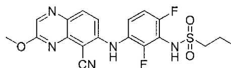
N -(3-(5-cyano-3-methoxyquinoxalin-6-ylamino)-2,6-difluorophenyl)propane-1-sulfonamide
