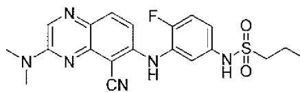
N -(3-(5-cyano-3-(dimethylamino)quinoxalin-6-ylamino)-4-fluorophenyl)propane-1-sulfonamide
