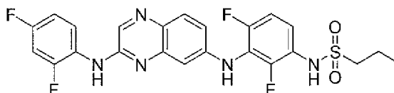
N1-(3-[[3-(2,4-difluoroanilino)-6-quinoxaliny]amino]-2,4-difluorophenyl)-1-propanesulfonamide
