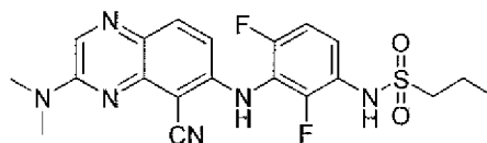
N -(3-(5-cyano-3-(dimethylamino)quinoxalin-6-ylamino)-2,4-difluorophenyl)propane-1-sulfonamide
