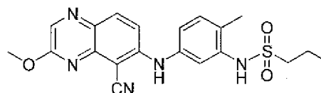
N -(5-(5-cyano-3-methoxyquinoxalin-6-ylamino)-2-methylphenyl)propane-1-sulfonamide
