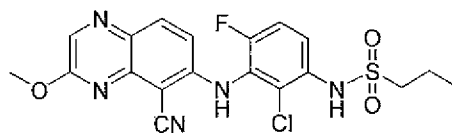
N -(2-chloro-3-(5-cyano-3-methoxyquinoxalin-6-ylamino)-4-fluorophenyl)propane-1-sulfonamide
