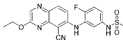
N -(3-(5-cyano-3-ethoxyquinoxalin-6-ylamino)-4-fluorophenyl)methanesulfonamide
