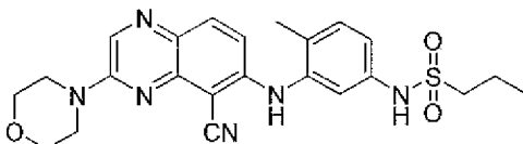
N -(3-(5-cyano-3-morpholinoquinoxalin-6-ylamino)-4-methylphenyl)propane-1-sulfonamide
