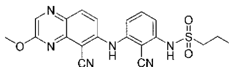
N -(2-cyano-3-(5-cyano-3-methoxyquinoxalin-6-ylamino)phenyl)propane-1-sulfonamide
