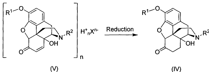
Scheme 8
