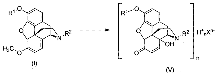
Scheme 14
