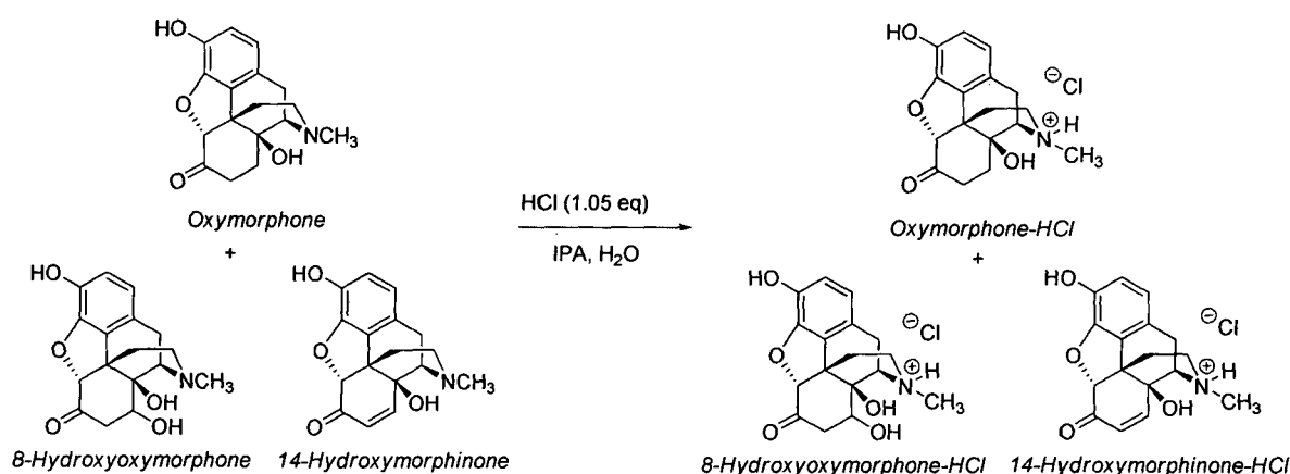
Scheme 22
