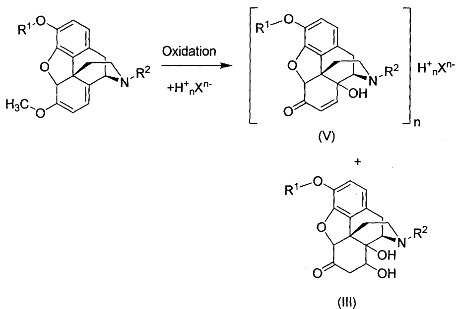
Scheme 16
