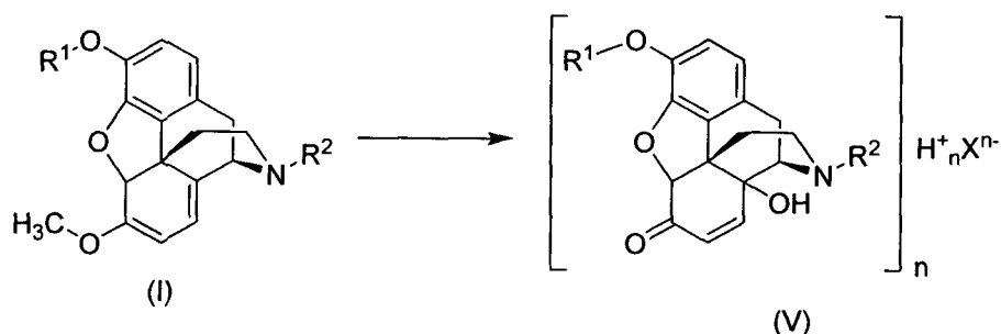
Scheme 9
