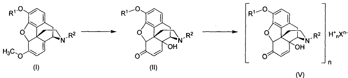
Scheme 10
