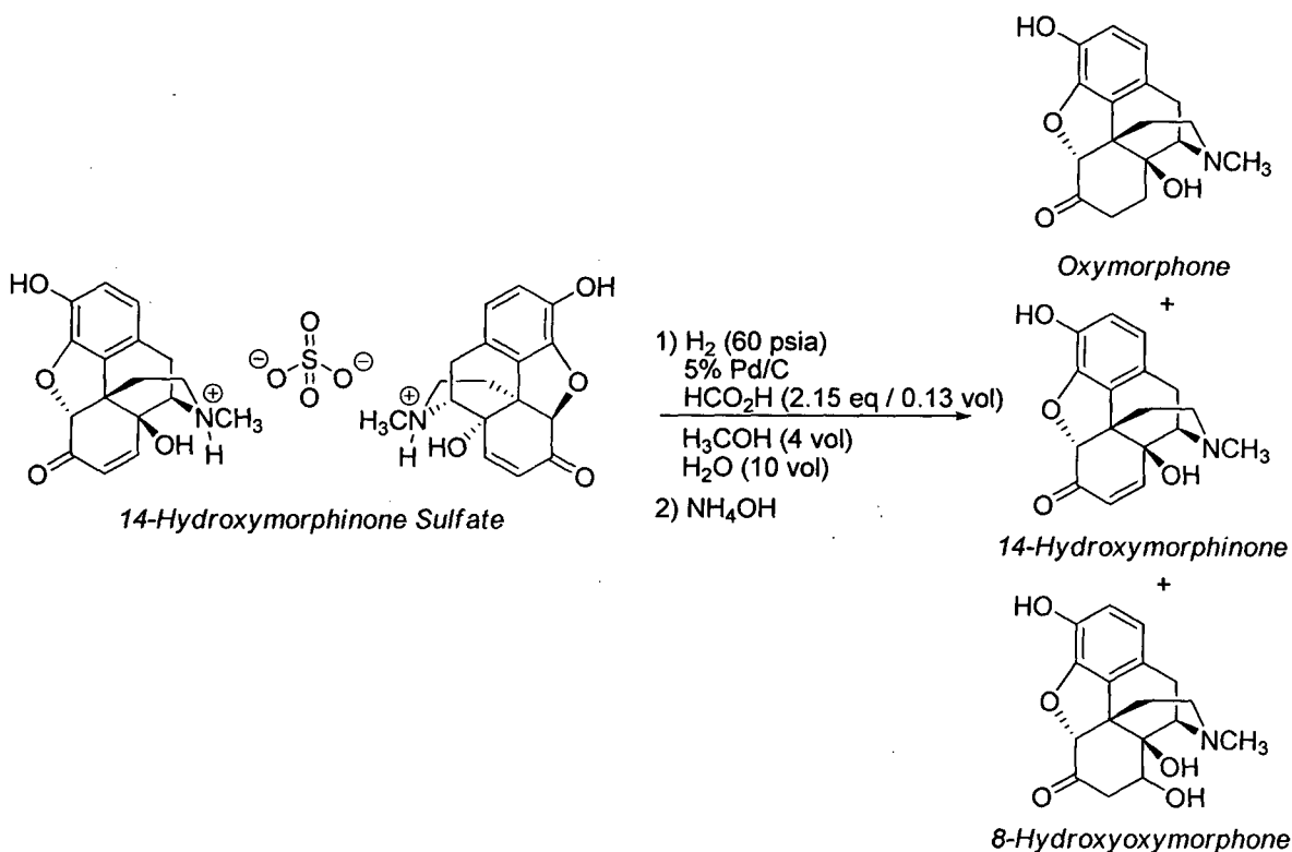
Scheme 20
