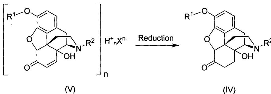
Scheme 17
