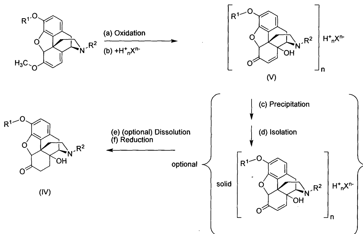
Scheme 19
