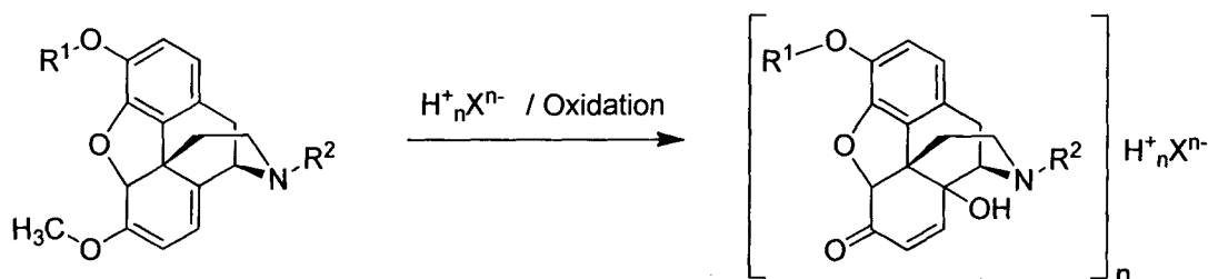
Scheme 12
