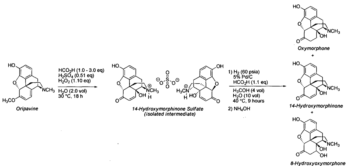
Scheme 21
