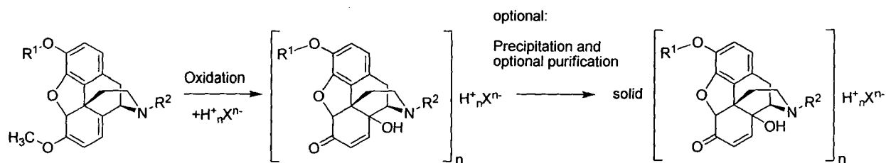
Scheme 15
