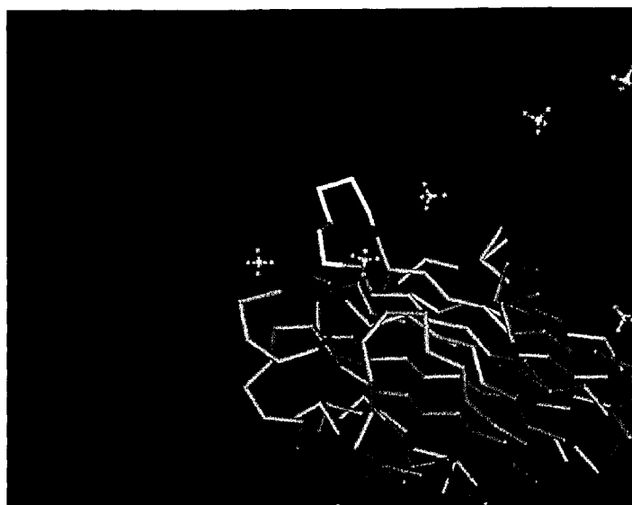
Figure 1: 1GWY Chain A, Crystal Structure Of The Water-S Of The Pore- Forming Cytolysin Sticholysin li
