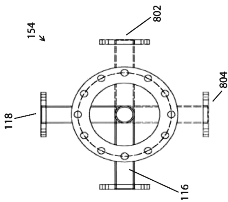
BALL SEPARATOR TOPVIEW
