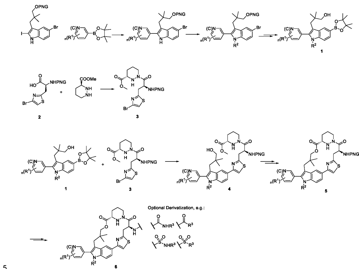
Scheme 1. General synthesis of macrocyclic esters
