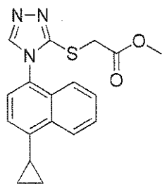
(Compound 2)
