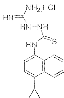
(Compound 13); and
