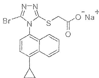
(Compound 4)
