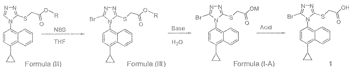
Scheme 6b
