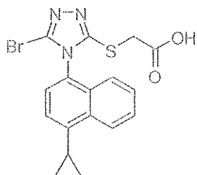
(Compound 1) or
