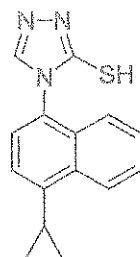
(Compound 5);
