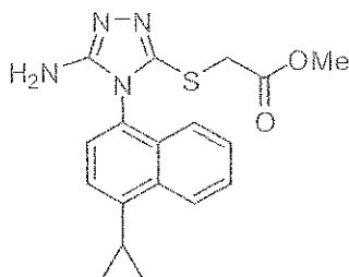
(Compound 12).
