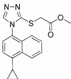
(Compound 2)
