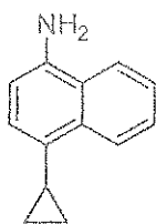
(Compound 8);
