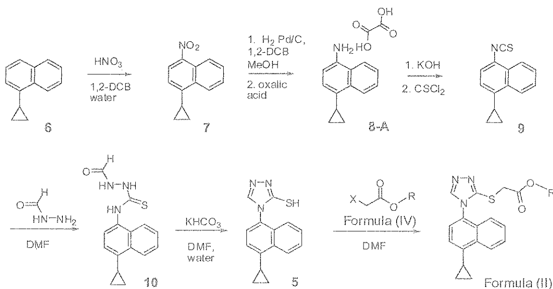
Scheme 5
