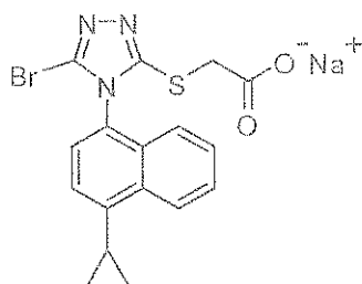
(Compound 4);
