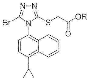
Formula (III);
