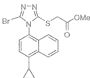
(Compound 3).
