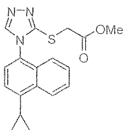
(Compound 2)
