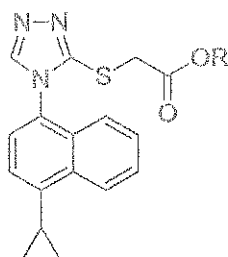
Formula (II);
