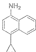
(Compound 8);
