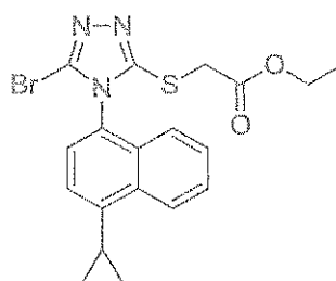
(Compound 3-A)
