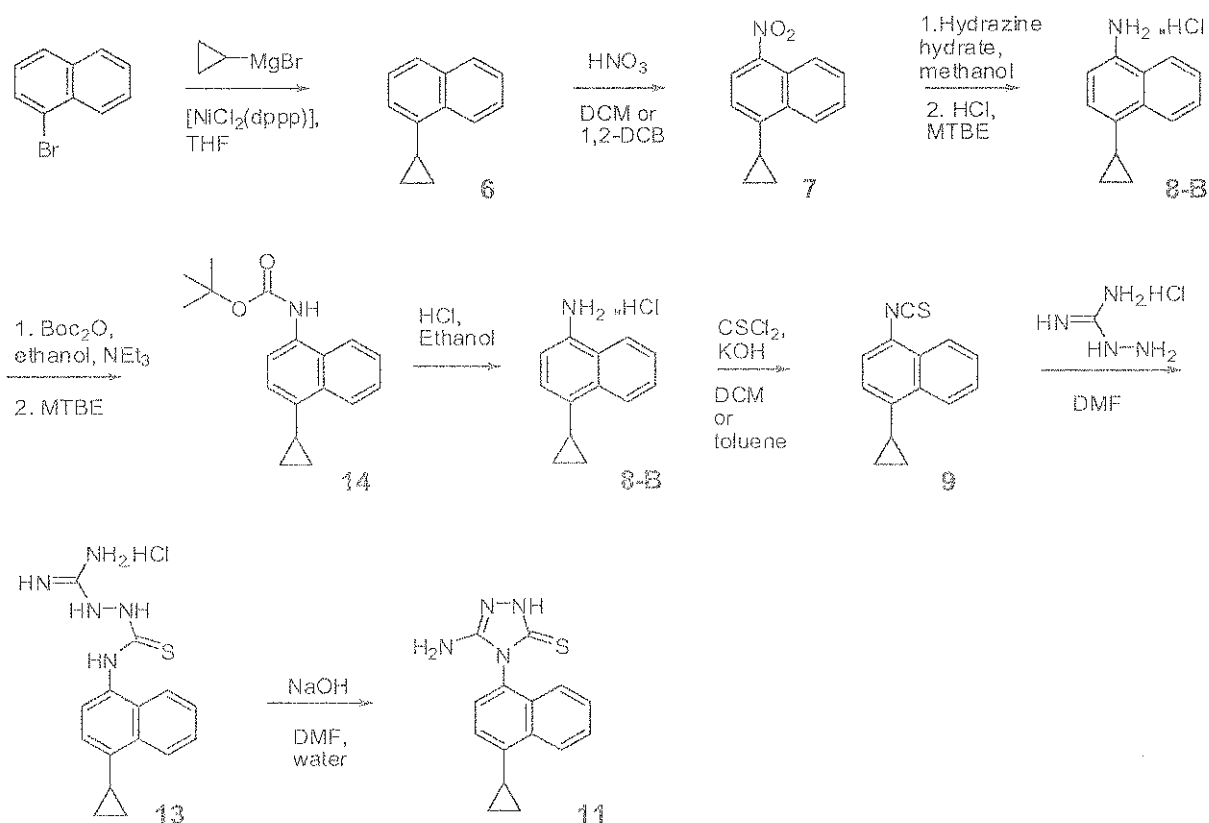
Scheme 3
