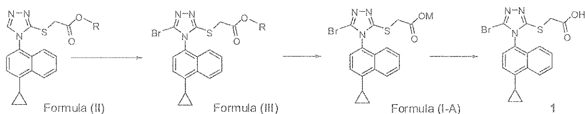
Scheme 6a
