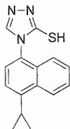
(Compound 5);
