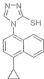
(Compound 5)
