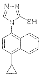
(Compound 5).
