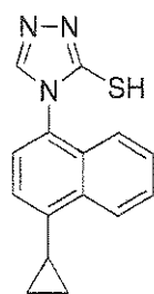
(Compound 5).
