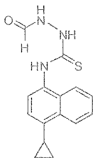
(Compound 10); and
