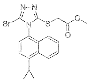
(Compound 3)
