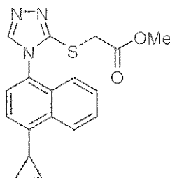
(Compound 2)
