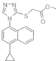
(Compound 2).
