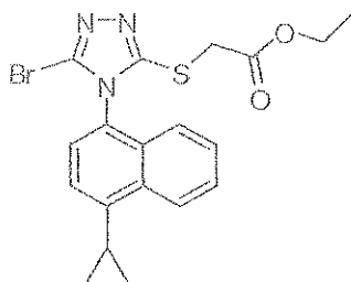
(Compound 3-A).
