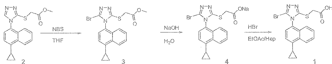
Scheme 7
