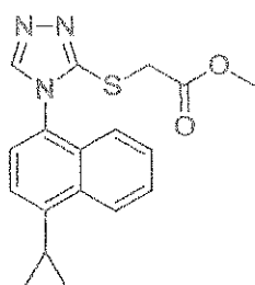
(Compound 2)
