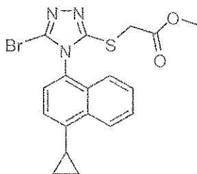
(Compound 3).
