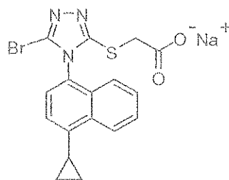
(Compound 4); and
