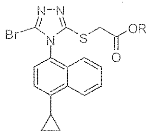
Formula (III);
