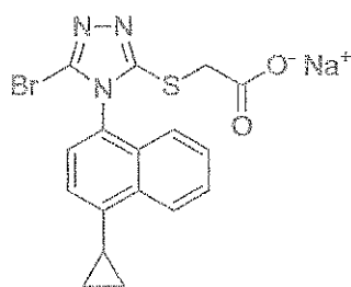
(Compound 4).
