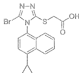
(Compound 1)
