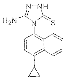
(Compound 11)
