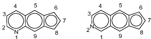
cyclopenta[g]quinolyl
