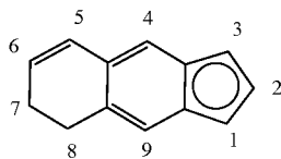
7,8-dihydro-cyclopenta[b]naphthalenyl.
