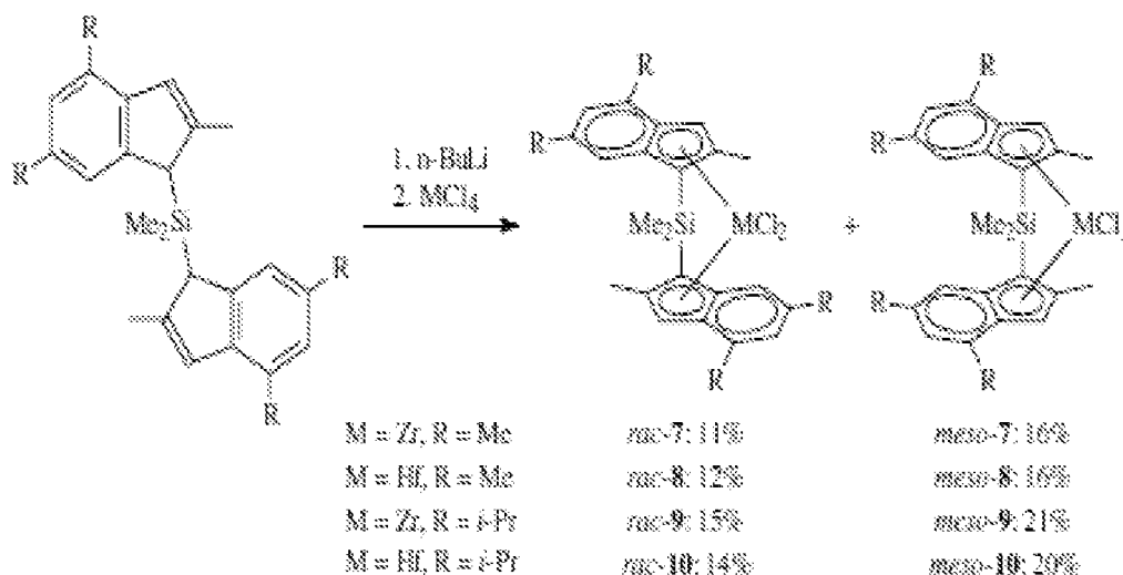
Scheme 6.
