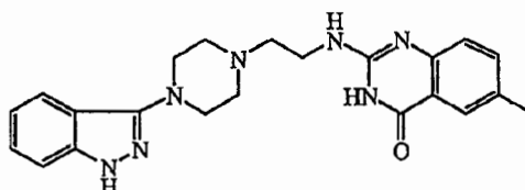
Compound 43
