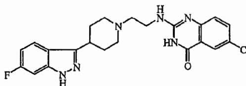
Compound 36
