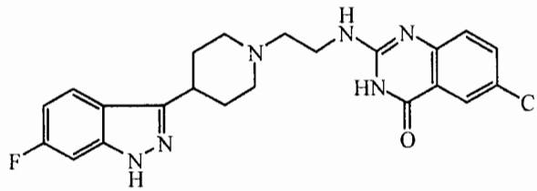
Compound 36
