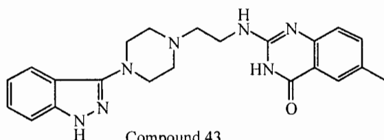
Compound 43
