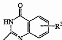
(b-3)
