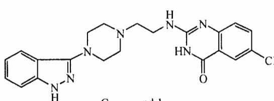
Compound 1
