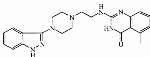
Compound 39
