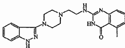
Compound 39
