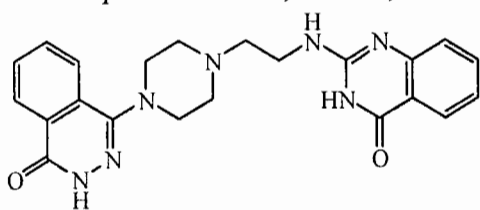
Compound 35
