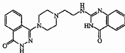
Compound 35
