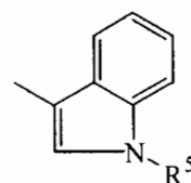
(b-8)
