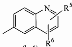
(b-4)
