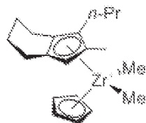
(Formula VIII)
