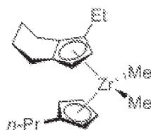
(Formula IX)
