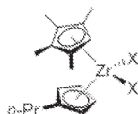
(Formula VII)
