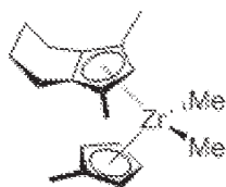
(Formula III)
