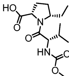
(2S,5S)-5-ethyl-1-((S)-2-(methoxycarbonylamino)-3-methylbutanoyl)pyrrolidine-2-carboxylic acid
