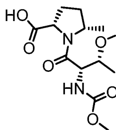
(2S,5S)-1-((2S,3R)-3-methoxy-2-(methoxycarbonylamino)butanoyl)-5-methylpyrrolidine-2-carboxylic acid
