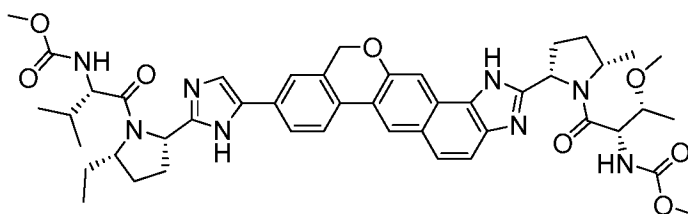
methyl{(2S,3R)-1-[(2S,5S)-2-(9-{2-[(2S,5S)-5-ethyl-1-{(2S)-2-[(methoxycarbonyl) amino]-3-methylbutanoyl}pyrrolidin-2-yl]-1H-imidazol-5-yl}-1,11-dihydroisochromeno[4',3':6,7]naphtho[1,2-d]imidazol-2-yl)-5-methylpyrrolidin-1-yl]-3-methoxy-1-oxobutan-2-yl}carbamate
