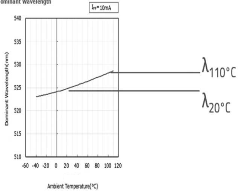
Ambient Temperature vs Dominant Wavelength
