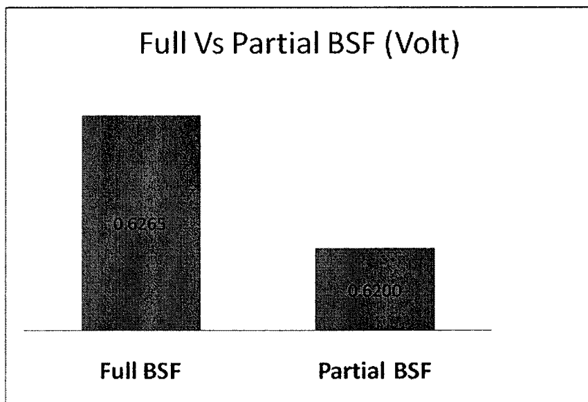
Fig. 14- Voc on 5"x5" mono-crystalline silicon solar cells
