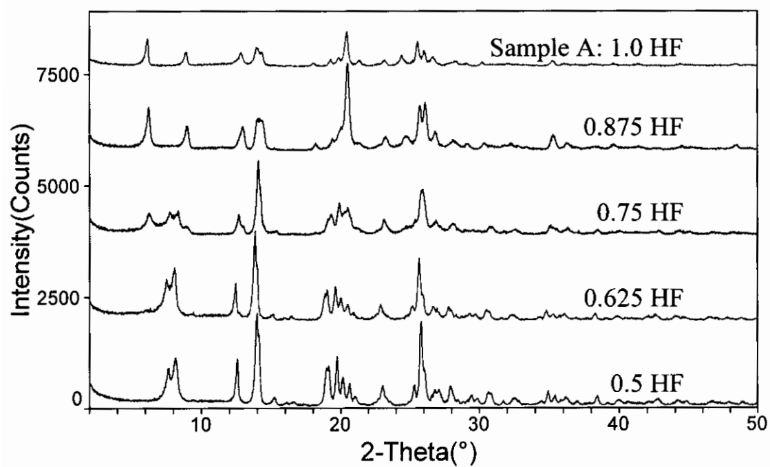
Figure 2. XRD's of Example 2 Products
