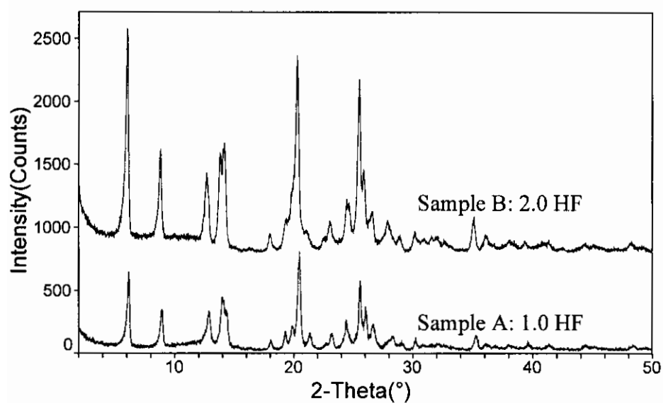
Figure 3. XRD's of Example 3 Products
