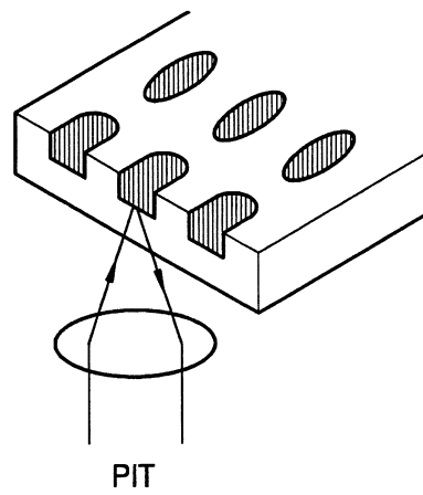
FIG. 3B (PRIOR ART)
