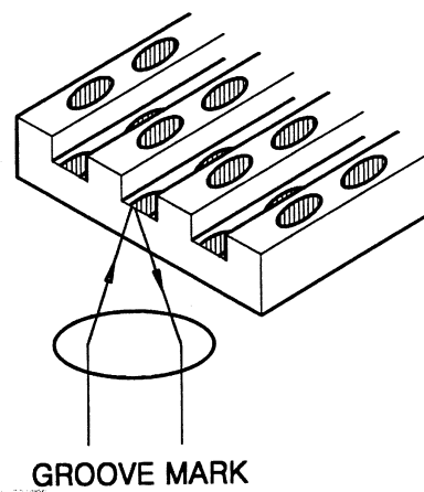
FIG. 3D (PRIOR ART)
