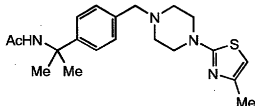
Example 139: N-(1-(4-((4-(4-methylthiazol-2-yl)piperazin-1-yl)methyl)phenyl)-1-methylethyl)acetamide
