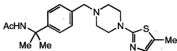
Example 139: N-(1-(4-((4-(4-methylthiazol-2-yl)piperazin-1-yl)methyl)phenyl)-1-methylethyl)acetamide
