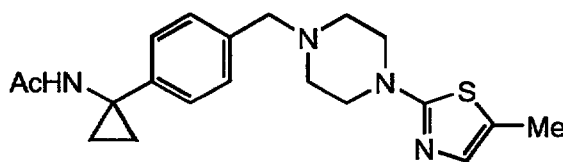
Example 141: N-(1-(4-((4-(5-methylthiazol-2-yl)piperazin-1-yl)methyl)phenyl)-1-methylethyl)acetamide
