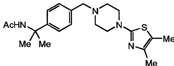
Example 140: N-(1-(4-((4-(4,5-dimethylthiazol-2-yl)piperazin-1-yl)methyl)phenyl)-1-methylethyl)acetamide
