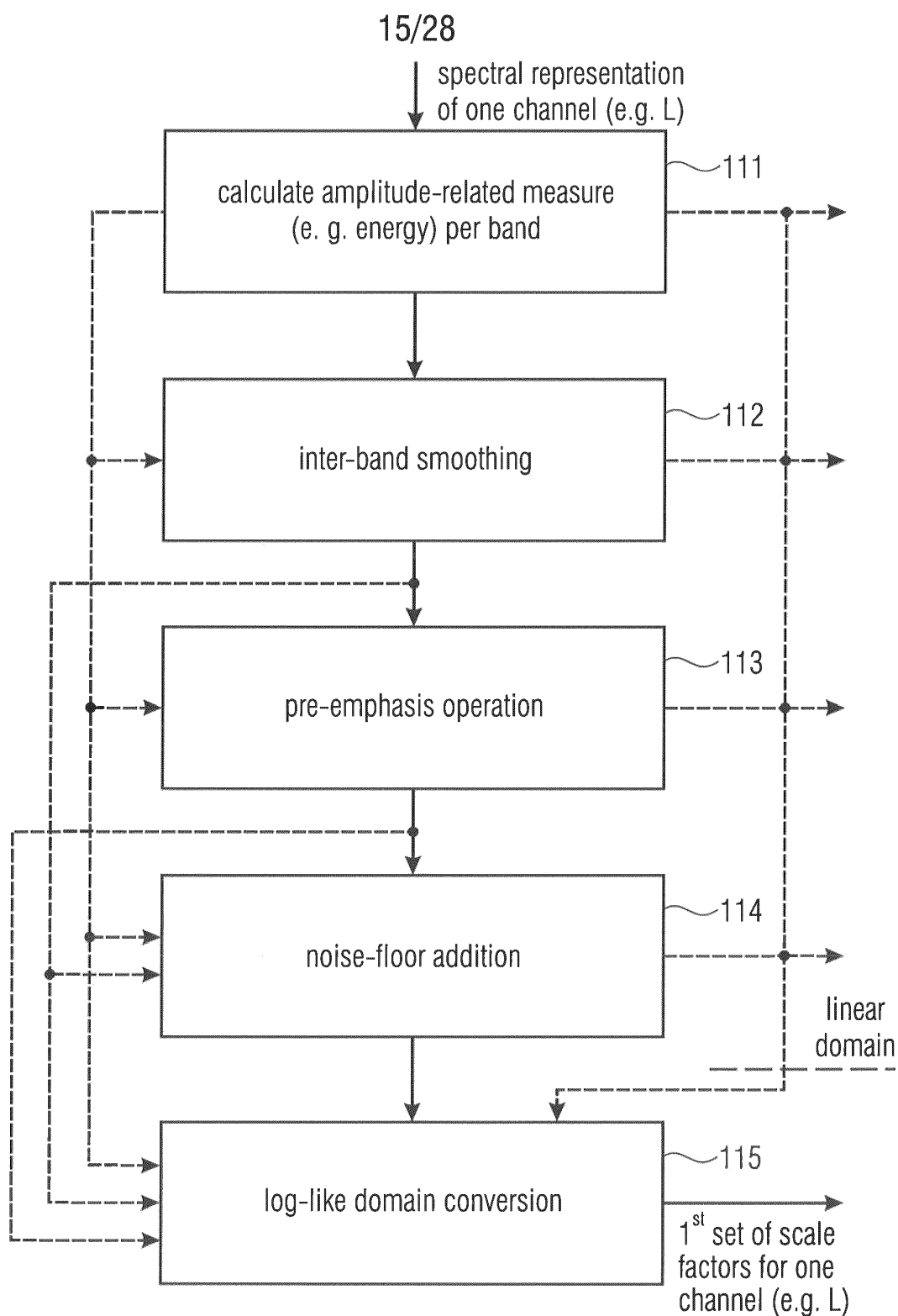
Fig. 12 (SCALE FACTOR CALCULATOR)
