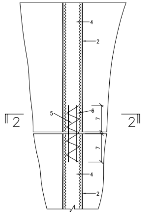
a final position of a connecting spiral reinforcement combination
