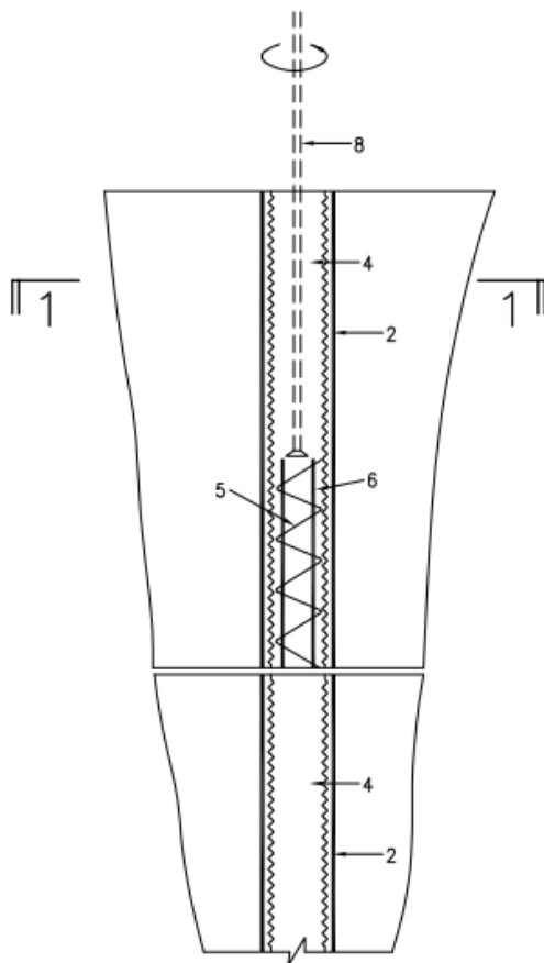
a start position of a connecting spiral reinforcement combination
