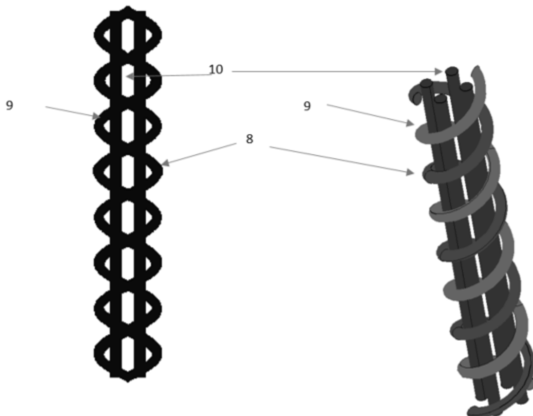
a double spiral reinforcement connector
