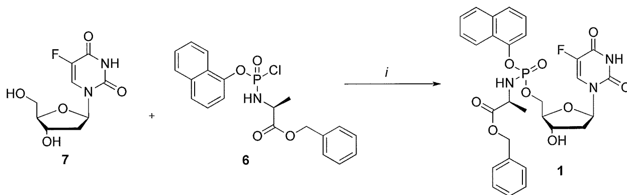
Scheme 3. Reagents and Conditions: ( i ) NMI, dry THF, 10 min., then phosphorochloridate ( 6 ), R.T., overnight.
