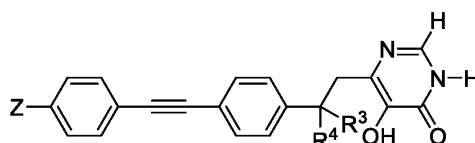
Formula (III).
