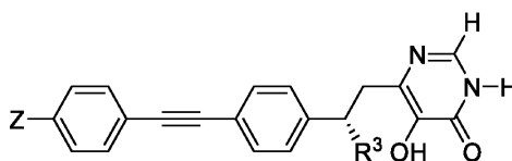
Formula (IVb).
