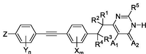
Formula (II).
