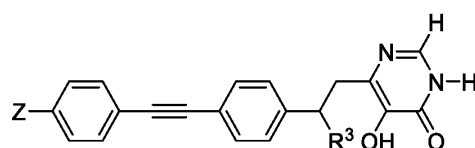
Formula (IV).
