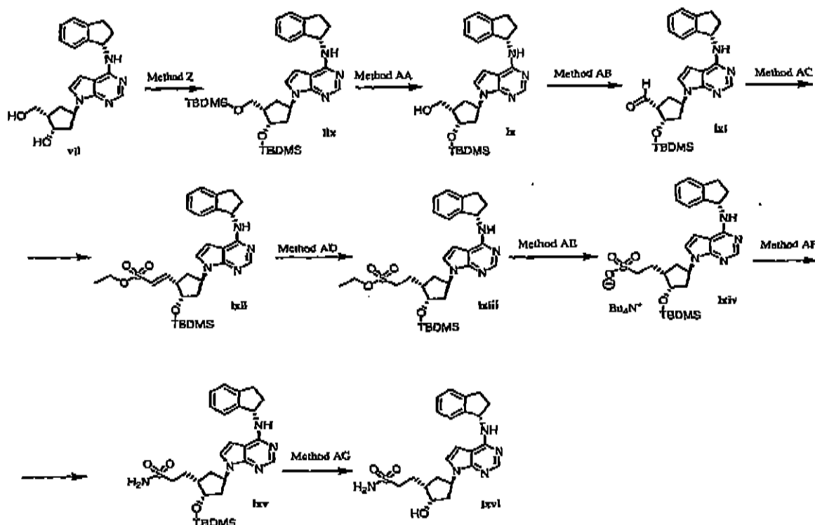
Scheme 11: Synthesis of 2-((1S,2S,4R)-4-4-((1S)-2,3-dihydro-1H-inden-1-ylamino)-7H-pyrrolo[2,3-d]pyrimidin-7-yl-2-hydroxycyclopentyl) ethanesulfonamide
