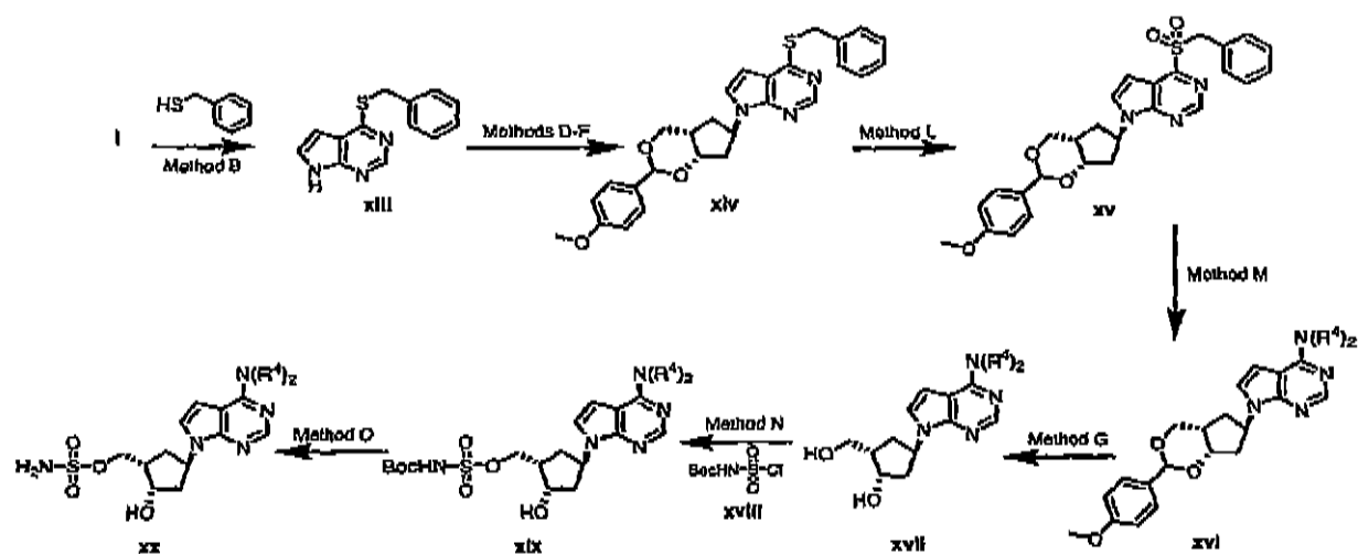
Scheme 2: Alternate route for the synthesis of 4- N -substituted ((1 S ,2 S ,4 R )-2-hydroxy-4-{7 R -pyrrolo[2,3- d ]pyrimidin-7-yl}cyclopentyl)methyl sulfamates
