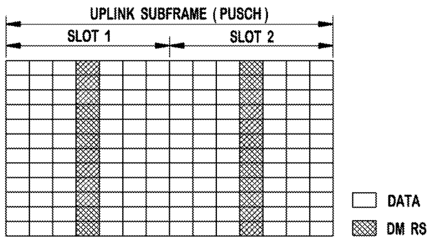
FIG. 9 (PRIOR ART)
