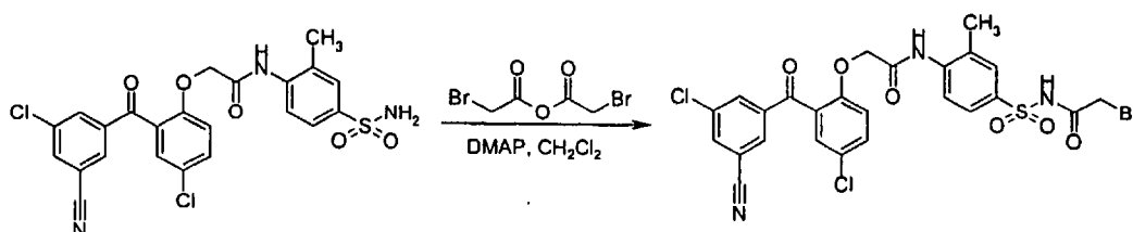
Scheme VII
