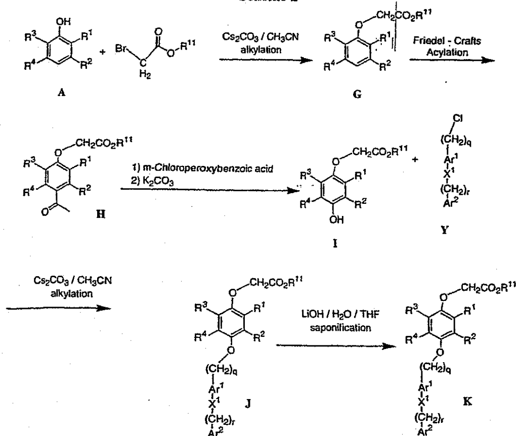
Scheme 2
