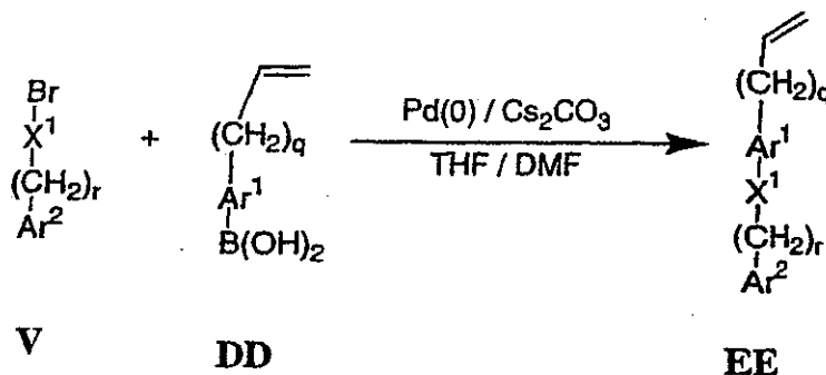
Scheme 9
