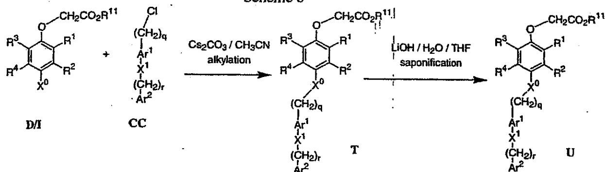
Scheme 6
