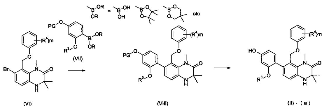
Synthetic Route 3
