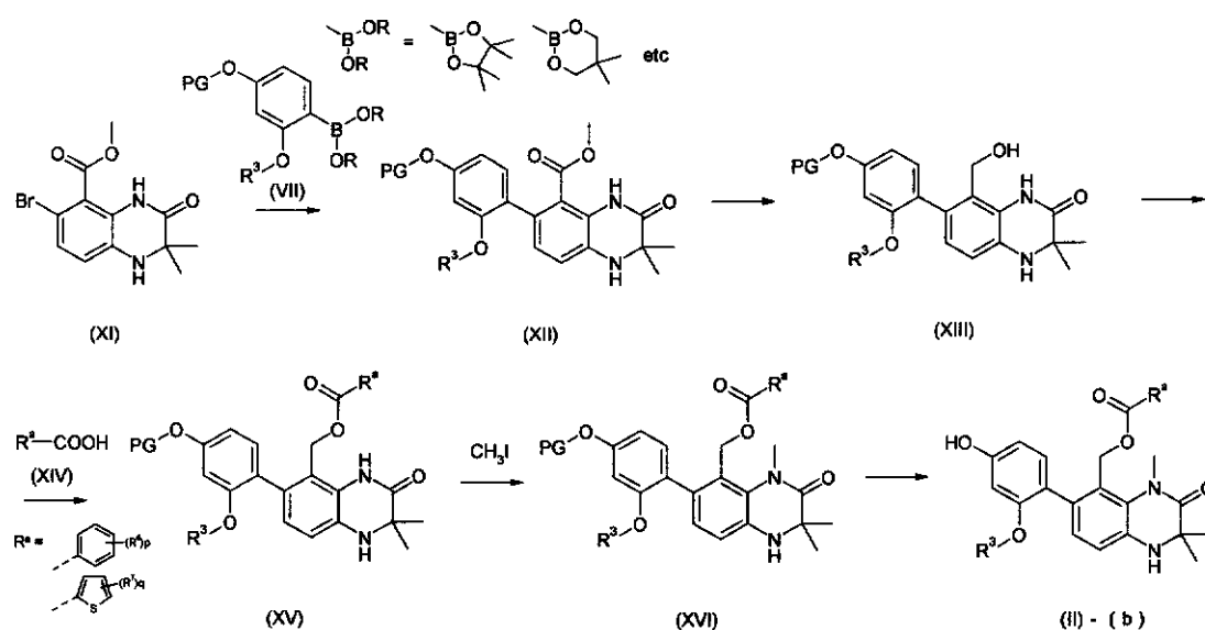
Synthetic Route 5
