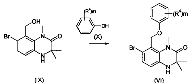
Synthetic Route 4
