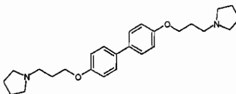
di-1,1'-{[(biphenyl-4,4'-diyl)bis[oxy(propan-1,3-diyl)]]}pyrrolidine
