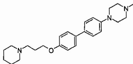
1-methyl-4-[4'-(3-piperidinopropoxy)biphenyl]piperazine
