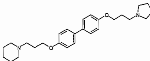
1-(3-([4'-(3-piperidinopropoxy)biphenyl-4-yloxy]propyl)pyrrolidine
