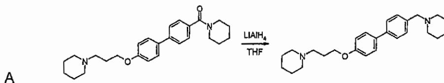
1-(3-[[4'-(piperidinomethyl)biphenyl-4-yl]oxy]propyl)piperidine
