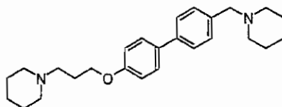
1-(3-[[4'-(piperidinomethyl)biphenyl-4-yl]oxy]propyl)piperidine
