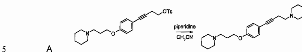
1-{3-[4-(4-Piperidinobut-1-yn-1-yl)phenoxy]propyl}piperidine
