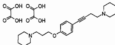
1-{3-[4-(4-Piperidinobut-1-yn-1-yl)phenoxy]propyl}piperidine
