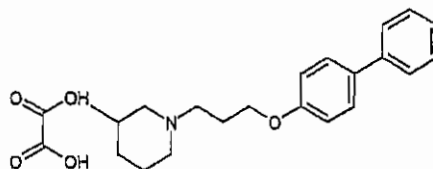
(RS)-1-{3-[(biphenyl-4-yl)oxy]propyl}-3-methylpiperidine, oxalate
