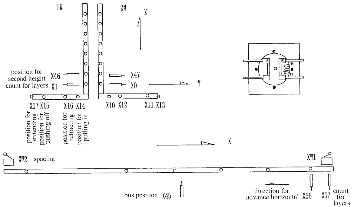
layout diagram of sensors on mechanical arms (47 points)
