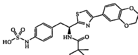
4-((S)-2-(4-(2,3-Dihydrobenzo[b][1,4]dioxin-6-yl)thiazol-2-yl)-2-pivalamidoethyl)phenylsulfamic acid
