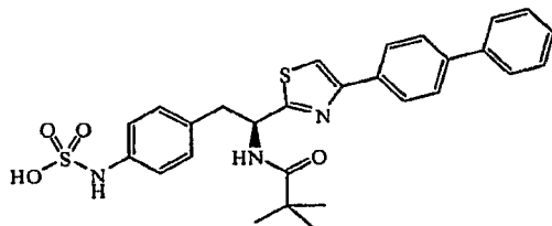
(S)-4-(2-(4-(Biphen-4-yl)thiazol-2-yl)-2-pivalamidoethyl)phenylsulfamic acid
