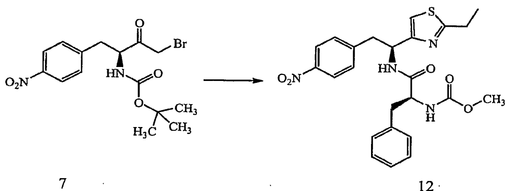
Scheme IV
