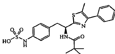
(S)-4-(2-(5-Methyl-4-phenylthiazol-2-yl)-2-pivalamidoethyl)phenylsulfamic acid
