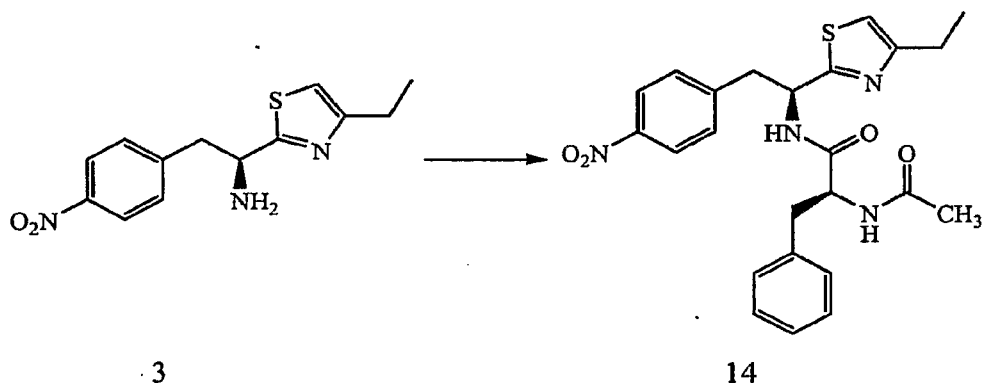
Scheme V
