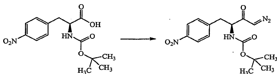
Scheme II
