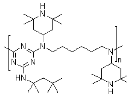
Charge Additive-6
