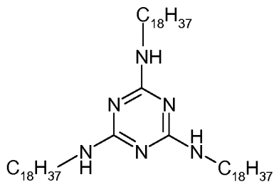
Charge Additive-5
