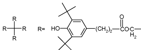
Charge Additive-14
