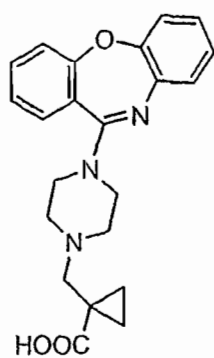
Compound 2
