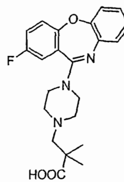
Compound 4
