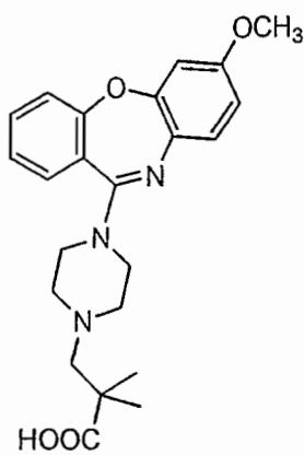
Compound 32
