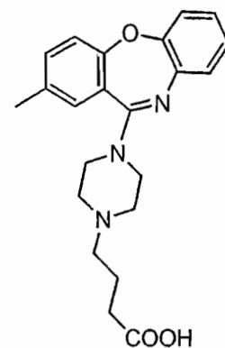
Compound 60
