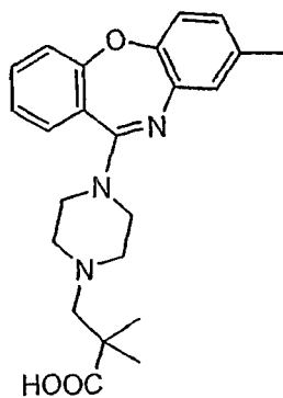
Compound 19
