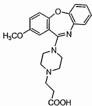
Compound 61
