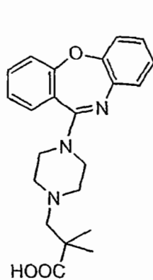
Compound 1
