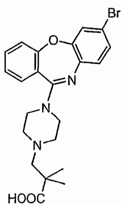
Compound 28
