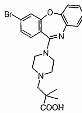
Compound 45
