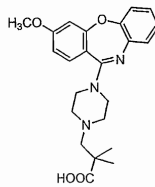
Compound 39
