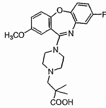
Compound 48
