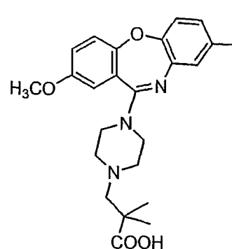
Compound 54
