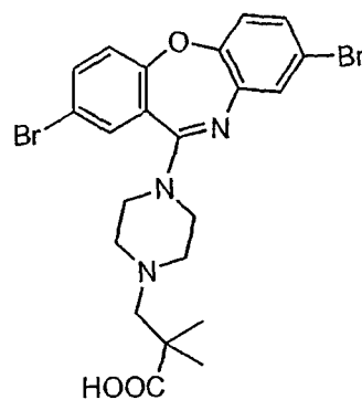
Compound 18
