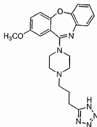
Compound 76
