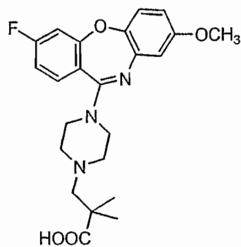
Compound 67
