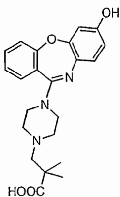
Compound 37
