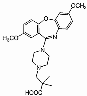
Compound 35
