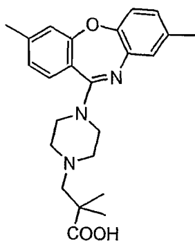
Compound 52
