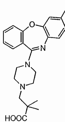
Compound 30
