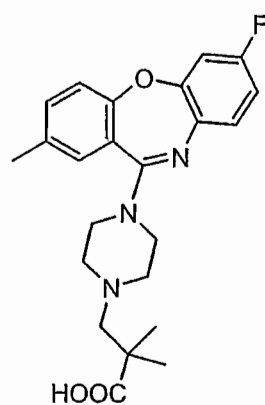
Compound 27
