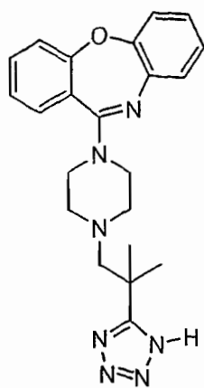
Compound 41
