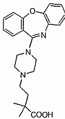
Compound 3
