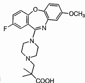
Compound 85
