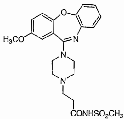
Compound 75
