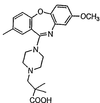
Compound 56
