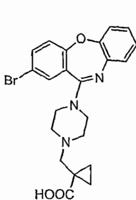
Compound 9
