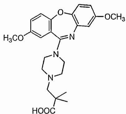
Compound 23
