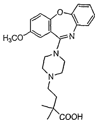
Compound 13
