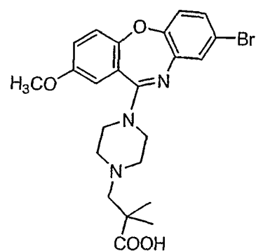
Compound 51
