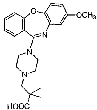
Compound 21
