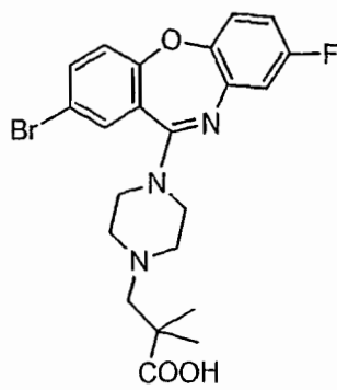
Compound 47
