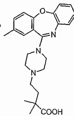
Compound 11
