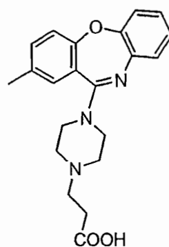
Compound 59
