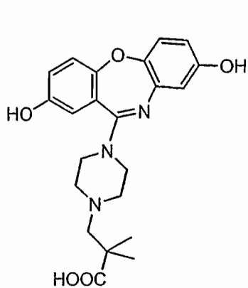
Compound 25
