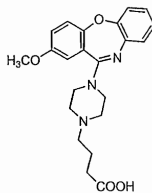
Compound 62
