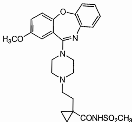
Compound 83
