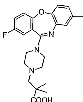
Compound 53
