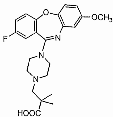
Compound 22
