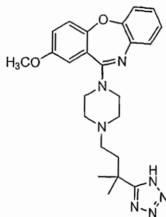
Compound 78
