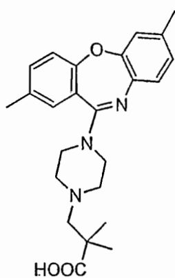
Compound 31
