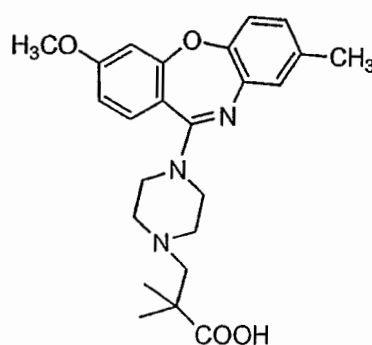
Compound 87
