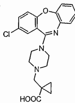
Compound 7
