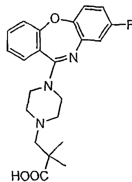
Compound 15
