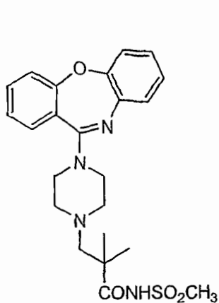
Compound 40
