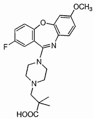
Compound 33
