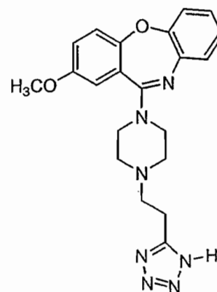
Compound 74
