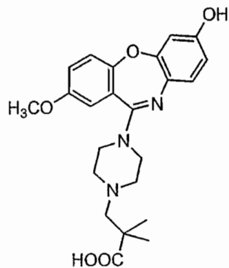
Compound 73
