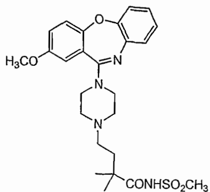
Compound 79
