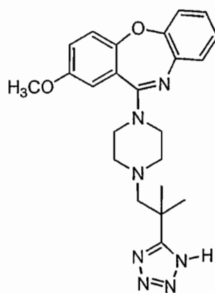
Compound 70
