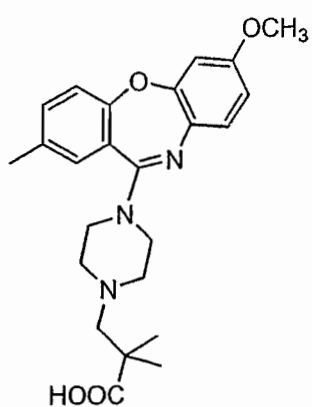
Compound 34
