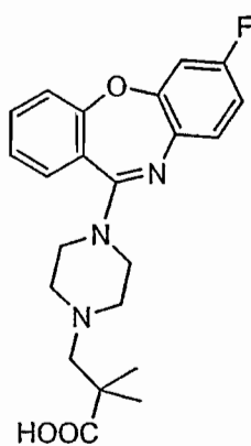
Compound 26
