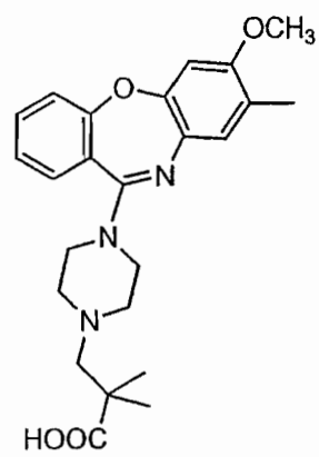
Compound 36
