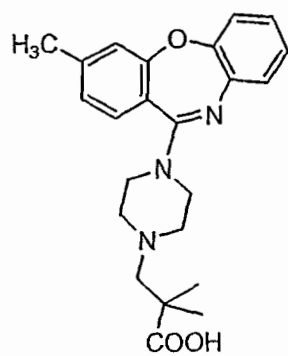
Compound 46
