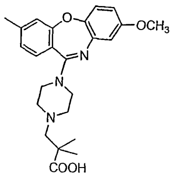
Compound 55
