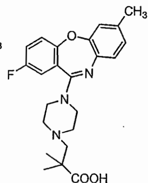
Compound 88
