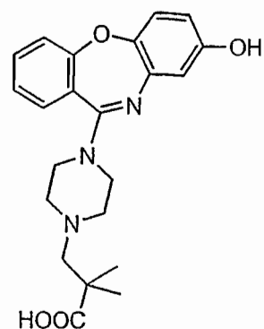
Compound 24
