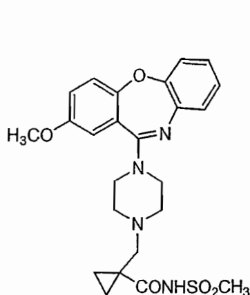
Compound 81
