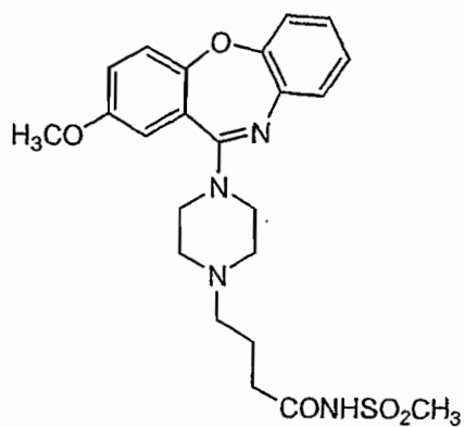
Compound 77
