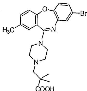
Compound 50
