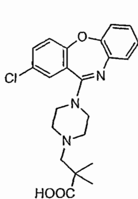
Compound 5
