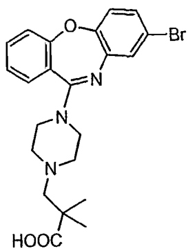
Compound 17
