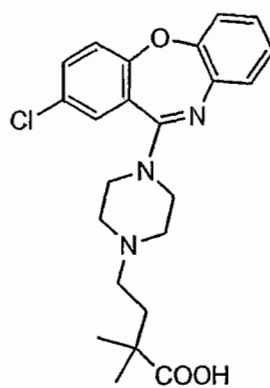
Compound 6
