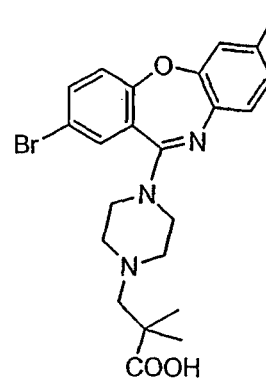
Compound 57
