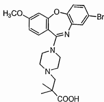
Compound 86
