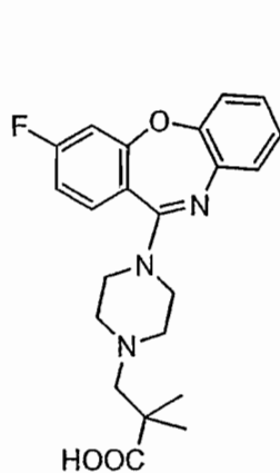
Compound 69
