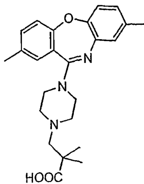
Compound 20
