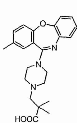
Compound 10
