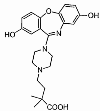
Compound 66
