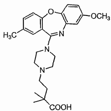
Compound 43
