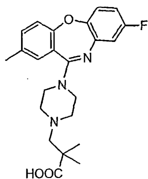
Compound 16
