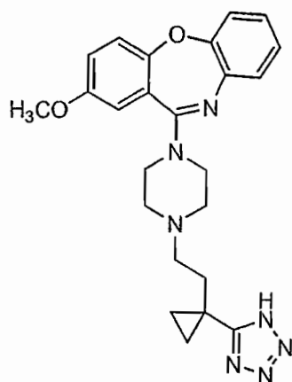
Compound 82
