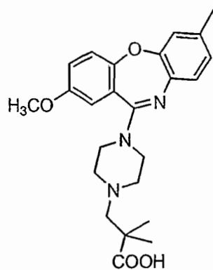
Compound 58
