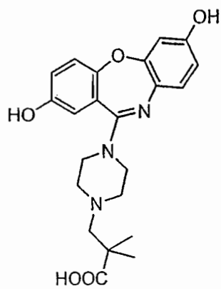
Compound 38
