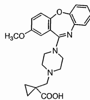
Compound 63
