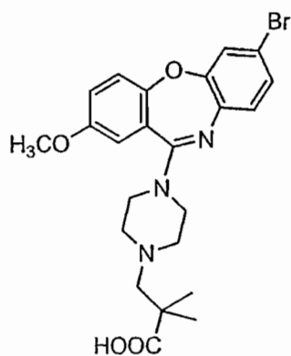
Compound 72
