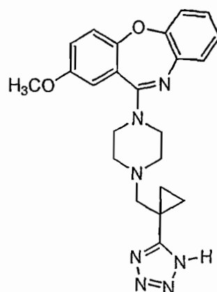
Compound 80
