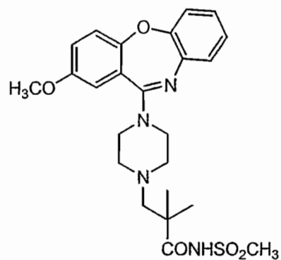
Compound 71
