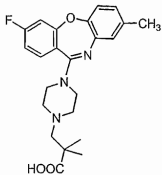
Compound 68
