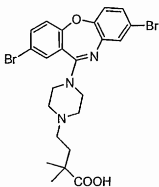
Compound 64
