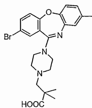
Compound 65
