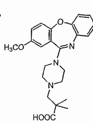
Compound 12
