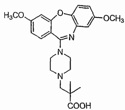
Compound 42
