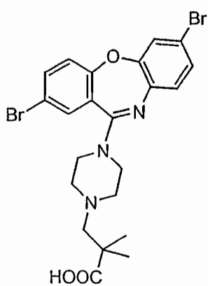
Compound 29
