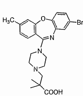
Compound 44
