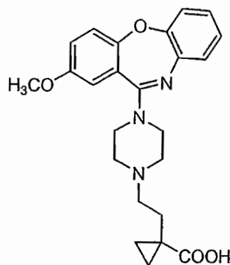
Compound 84
