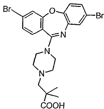
Compound 49
