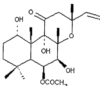
Structure of Isoforskolin
