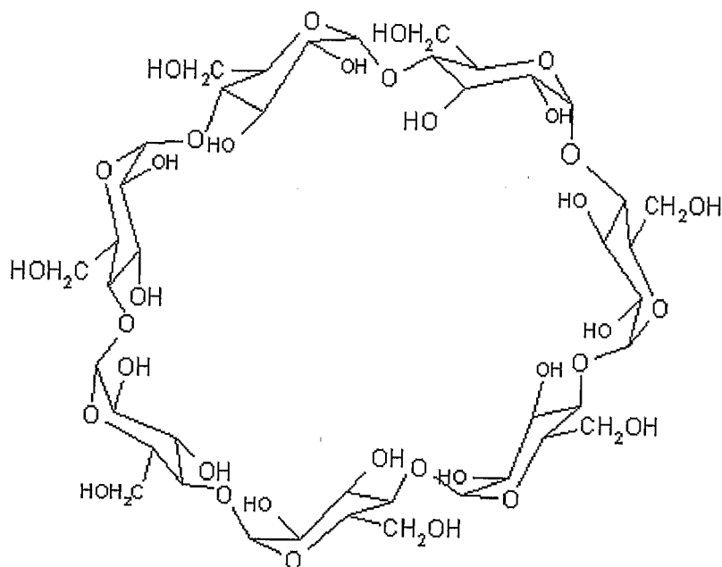
Structure of Beta-cyclodextrin
