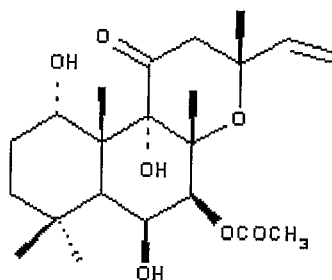
Structure of Forskolin
