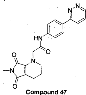
Compound 47
