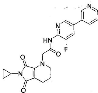
Compound 107
