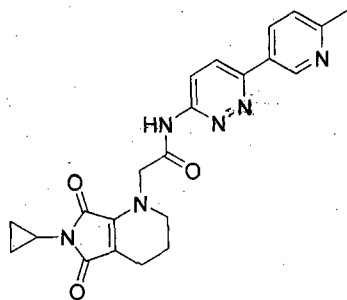
Compound 86
