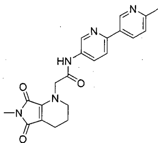
Compound 24
