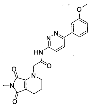
Compound 32
