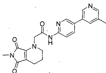
Compound 148
