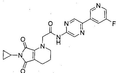
Compound 142
