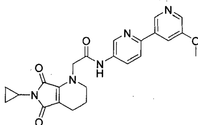
Compound 144
