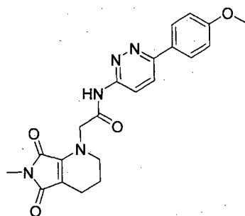
Compound 31
