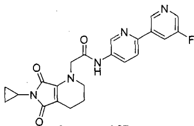
Compound 87
