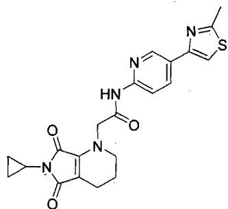
Compound 15
