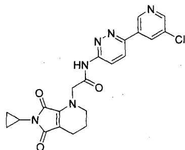
Compound 58
