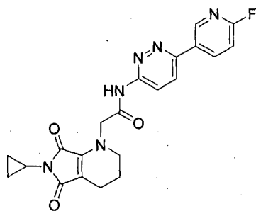
Compound 69
