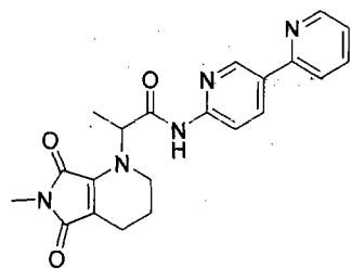
Compound 17
