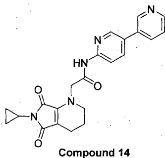
Compound 14
