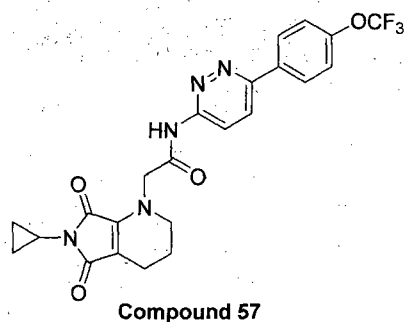
Compound 57
