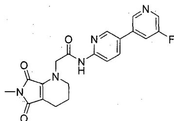
Compound 143
