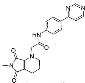
Compound 73
