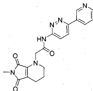
Compound 25
