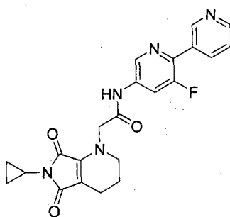
Compound 109
