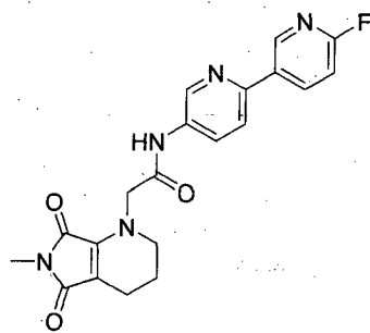
Compound 108
