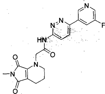
Compound 72
