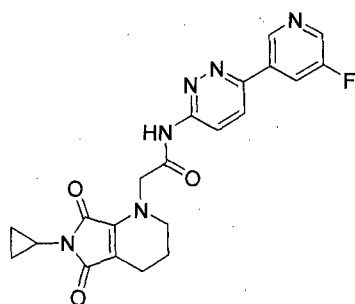
Compound 52
