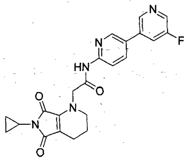
Compound 106
