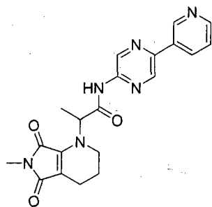
Compound 23
