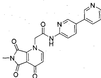
Compound 63
