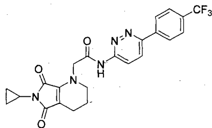
Compound 51
