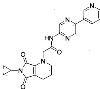
Compound 26
