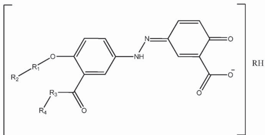
Formula XIII
