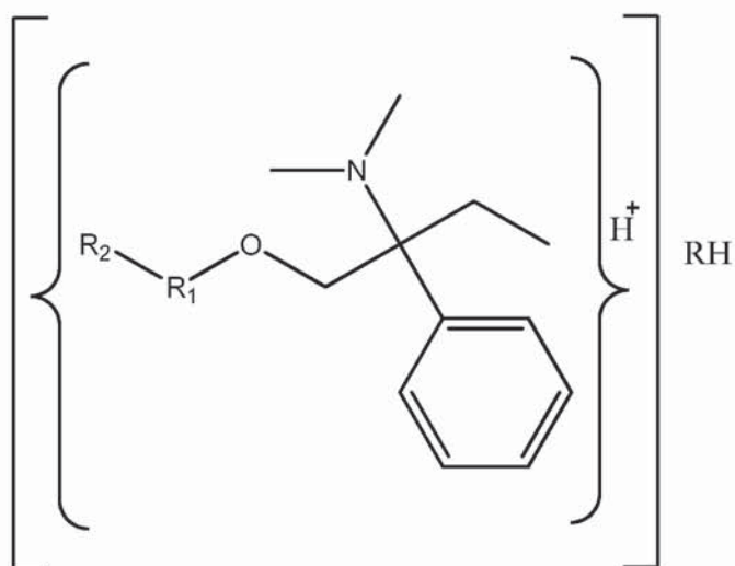
Formula IX
