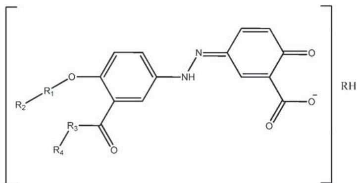
Formula XIV
