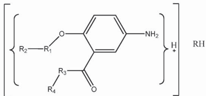
Formula VII
