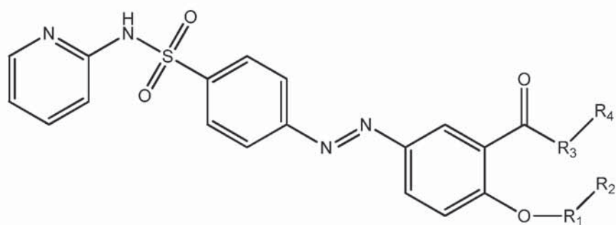
Formula III
