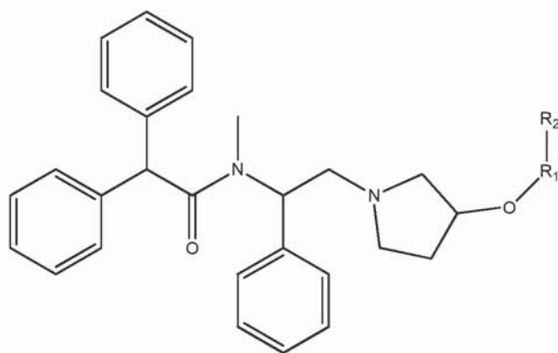
Formula VI
