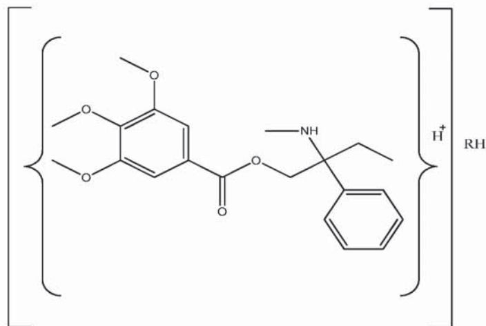
Formula XI
