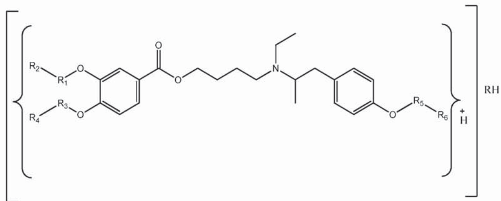
Formula X
