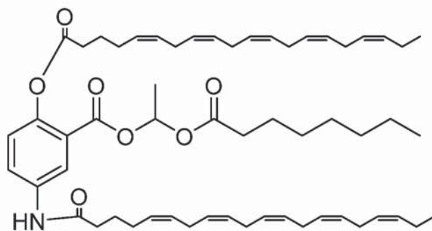
1-(octanoyloxy)ethyl 5-(((5Z,8Z,11Z,14Z,17Z)-icosa-5,8,11,14,17-pentaenamido)-2-(((5Z,8Z,11Z,14Z,17Z)-icosa-5,8,11,14,17-pentaenoyl)oxy)benzoate.
