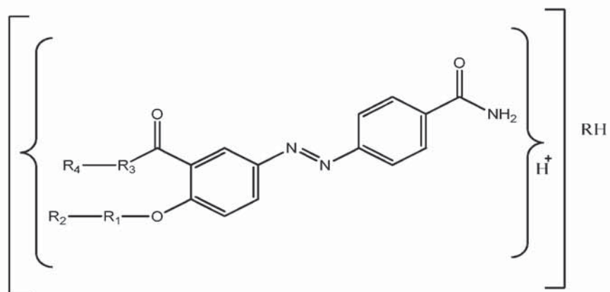
Formula VIII
