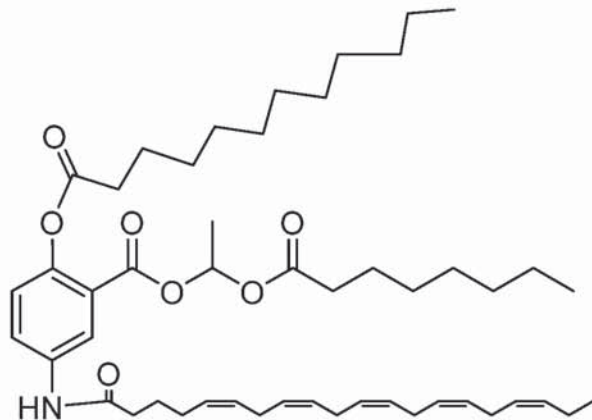
1-(octanoyloxy)ethyl 2-(dodecanoyloxy)-5-(((5Z,8Z,11Z,14Z,17Z)-icosa-5,8,11,14,17-pentaenamido)benzoate.
