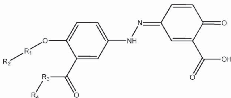
Formula XV
