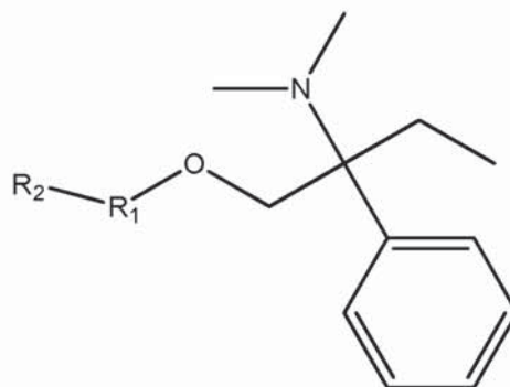
Formula V
